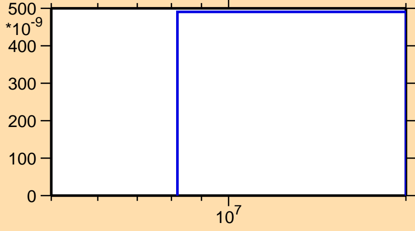
\sigma vs. E for ^{236}\text{Np}(n,nd)
