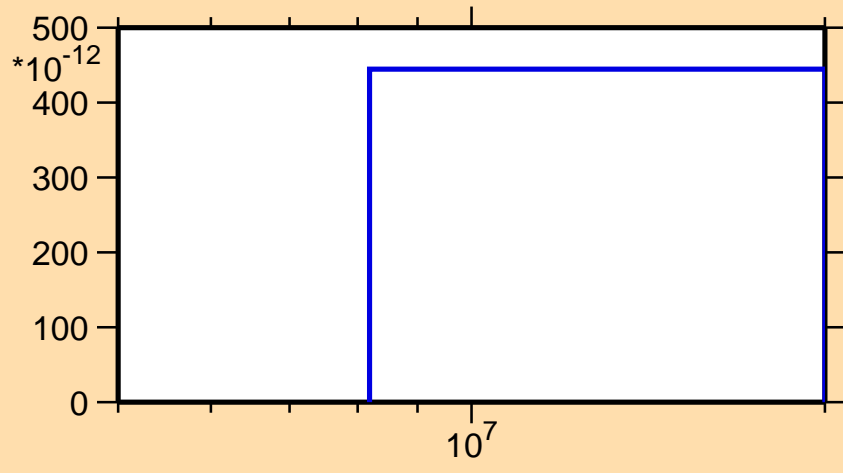
\sigma vs. E for ^{236}\text{Np}(n,p\alpha)
