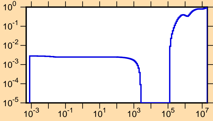
\mu vs. E for ^{238}\text{Np}(\text{mt251})
