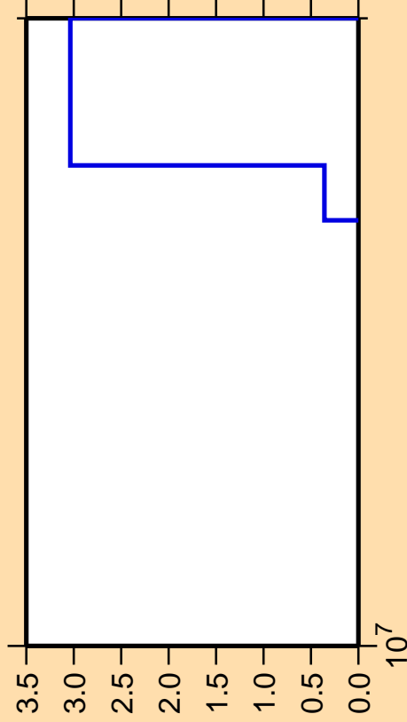
\Delta\sigma/\sigma vs. E for ^{238}\text{Np}(\text{mt } 45)
