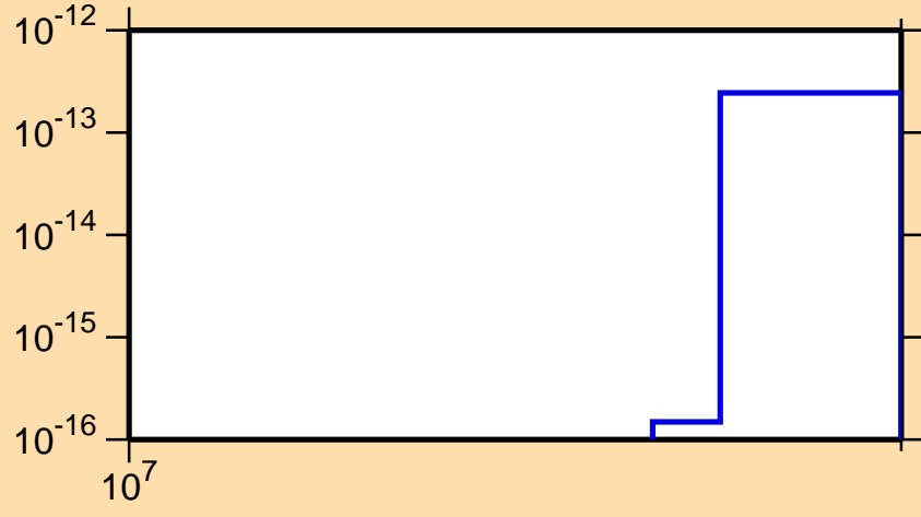
\sigma vs. E for ^{238}\text{Np} (mt 11)
