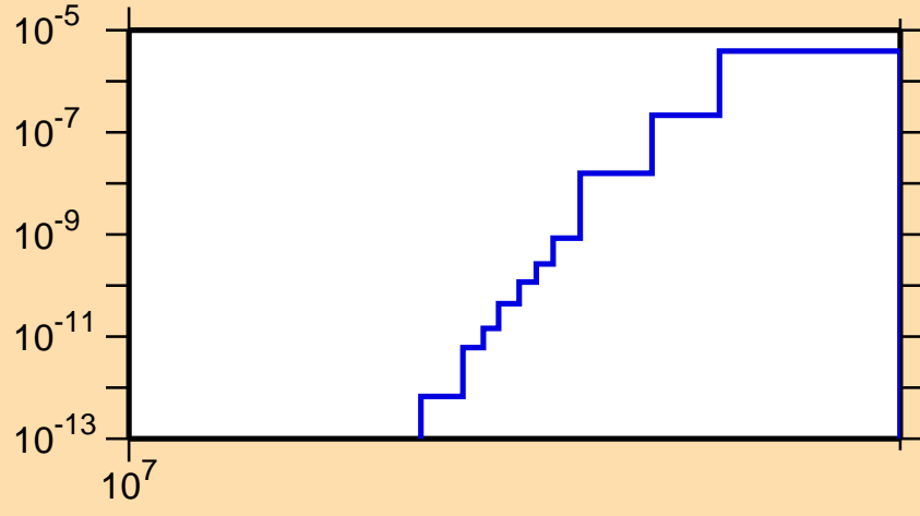
\sigma vs. E for ^{238}\text{Np}(n,nt)
