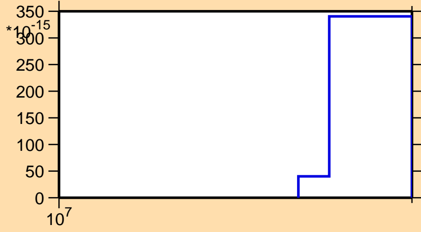
\sigma vs. E for ^{238}\text{Np}(\text{mt } 45)
