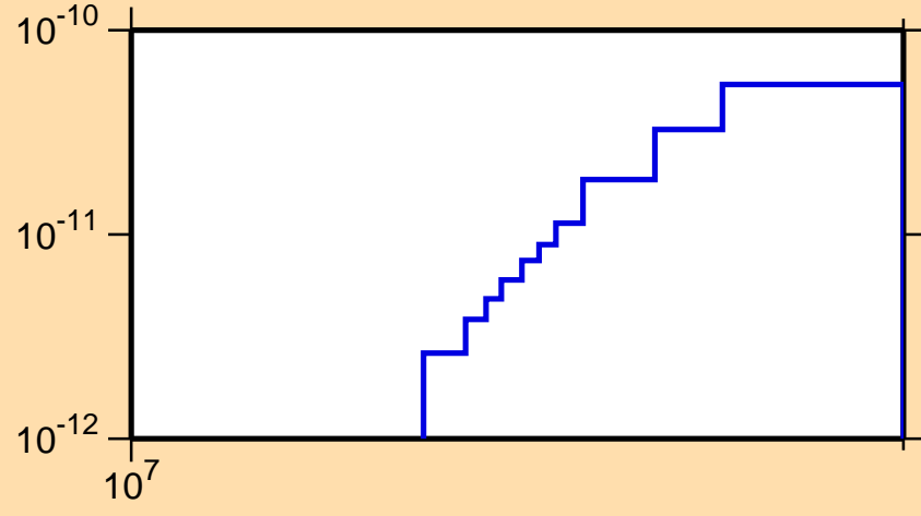
\sigma vs. E for ^{238}\text{Np}(n,p\alpha)
