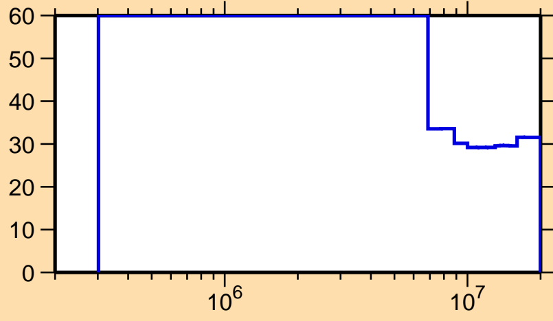
\Delta\sigma/\sigma vs. E for ^{238}\text{Np}(n,n\text{cont.})
