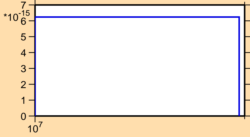
\sigma vs. E for ^{238}\text{Np} (mt 45)
