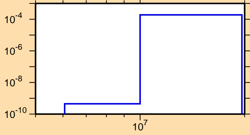
\sigma vs. E for ^{238}\text{Np}(n,d)
