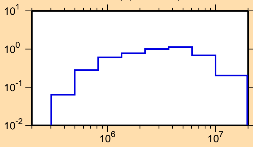
\sigma vs. E for ^{238}\text{Np}(n,n\text{cont.})
