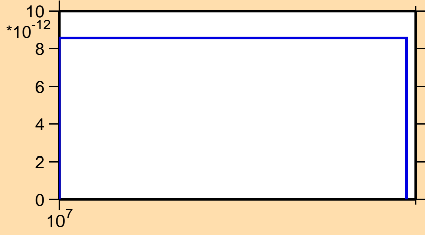
\sigma vs. E for ^{238}\text{Np}(n,p\alpha)
