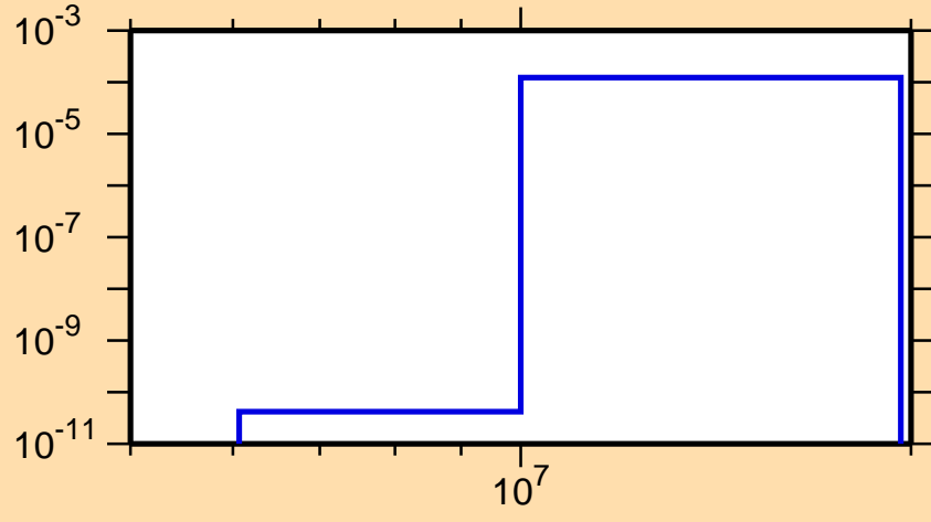
\sigma vs. E for ^{238}\text{Np}(n,np)
