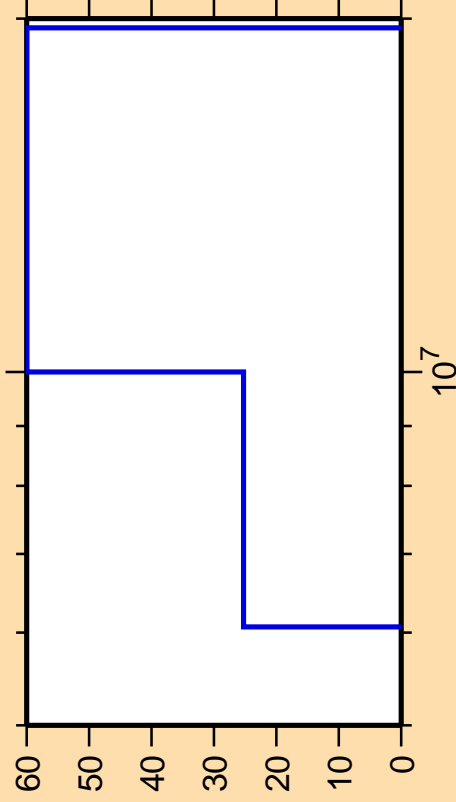
\Delta\sigma/\sigma vs. E for ^{238}\text{Np}(n,np)
