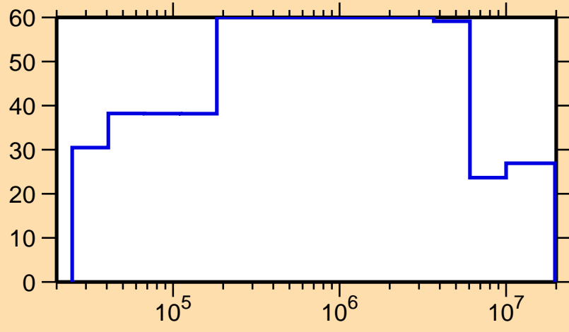
\Delta\sigma/\sigma vs. E for ^{238}\text{Np}(n,f)
