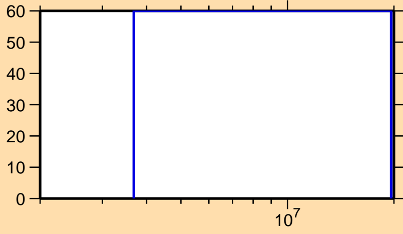
\Delta\sigma/\sigma vs. E for ^{238}\text{Np}(n,2n)
