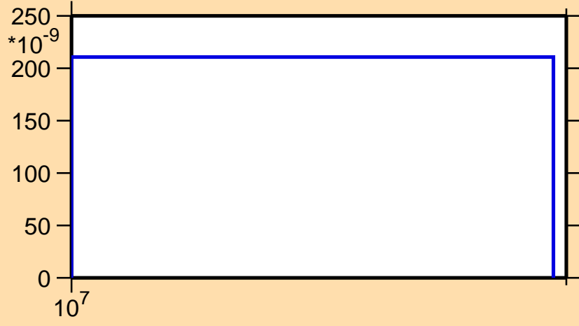
\sigma vs. E for ^{238}\text{Np}(n,nd)
