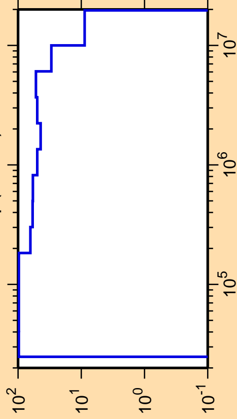
\Delta\sigma/\sigma vs. E for ^{238}\text{Np}(n,\text{inel.})
