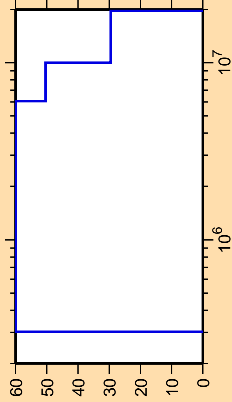
\Delta\sigma/\sigma vs. E for ^{238}\text{Np}(n,n_{\text{cont}}) .
