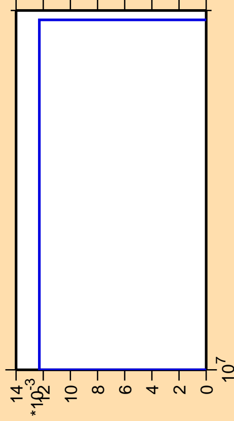
\Delta\sigma/\sigma vs. E for ^{238}\text{Np} (mt 11)
