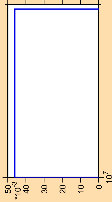
\Delta\sigma/\sigma vs. E for ^{238}\text{Np} (mt 45)
