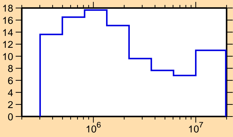
\Delta\sigma/\sigma vs. E for ^{238}\text{Np}(n,\text{tot.})
