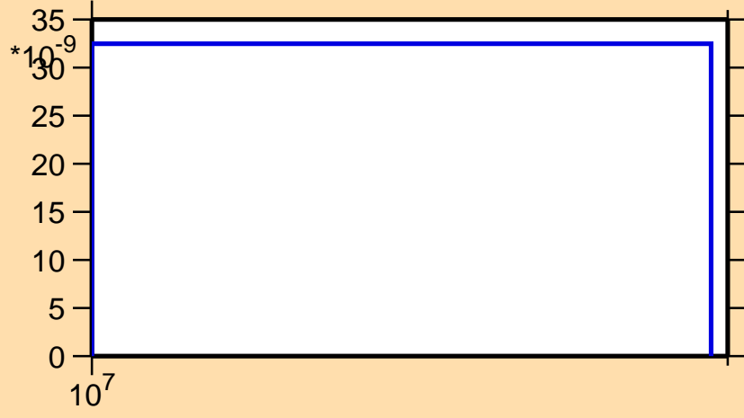
\sigma vs. E for ^{238}\text{Np}(n,2np)
