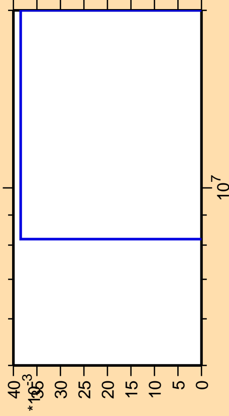
\Delta\sigma/\sigma vs. E for ^{238}\text{Np}(\text{mt } 45)
