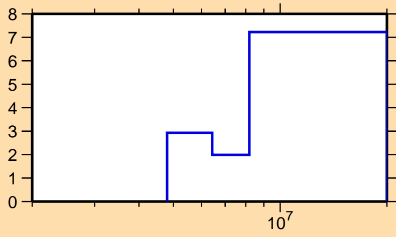
\Delta\sigma/\sigma vs. E for ^{238}\text{Np}(n,\text{el.})
