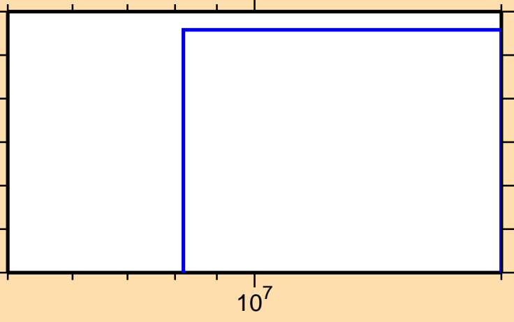
\sigma vs. E for ^{238}\text{Np}(n,2np)
