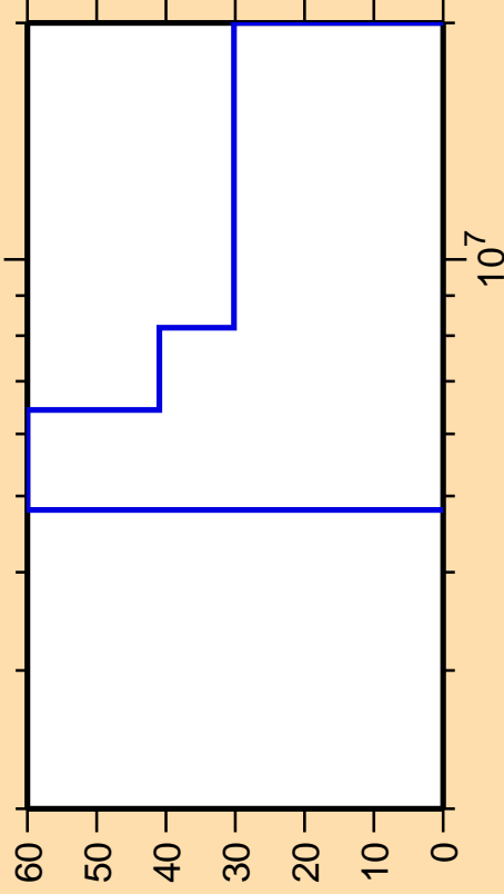
\Delta\sigma/\sigma vs. E for ^{238}\text{Np}(n,ncont.)
