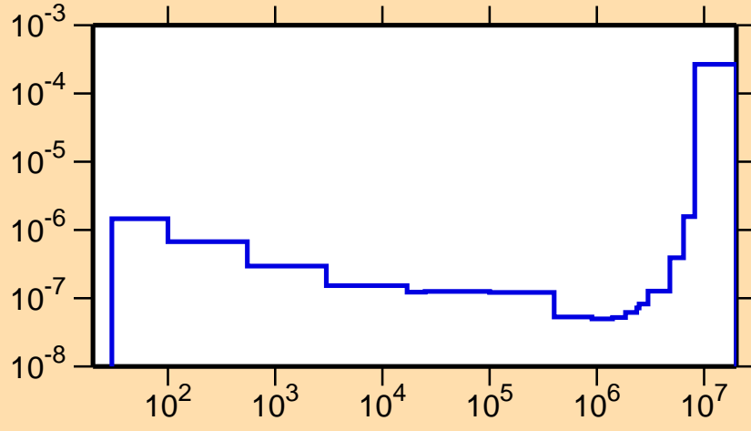
\sigma vs. E for ^{238}\text{Np}(n,\alpha)
