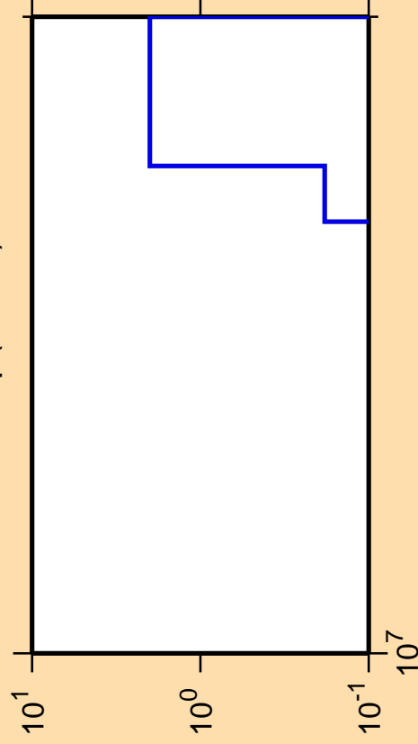
\Delta\sigma/\sigma vs. E for ^{239}\text{Np} (mt 45)
