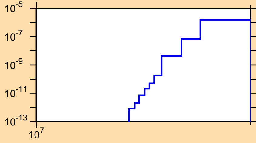
\sigma vs. E for ^{239}\text{Np}(n,nd)
