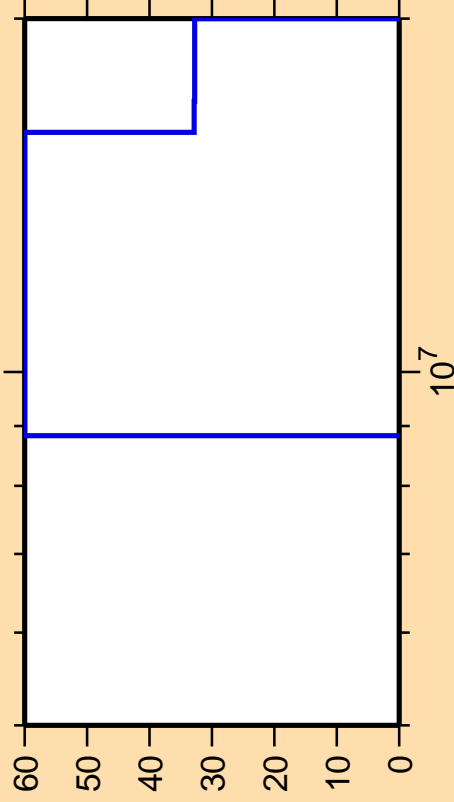
\Delta\sigma/\sigma vs. E for ^{239}\text{Np}(n,t)
