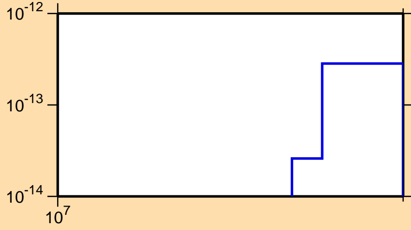
\sigma vs. E for ^{239}\text{Np} (mt 45)
