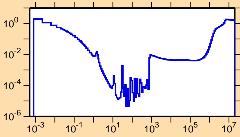
\sigma vs. E for ^{239}\text{Np}(n,f)
