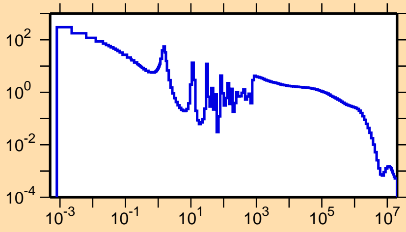
\sigma vs. E for ^{239}\text{Np}(n,\gamma)
