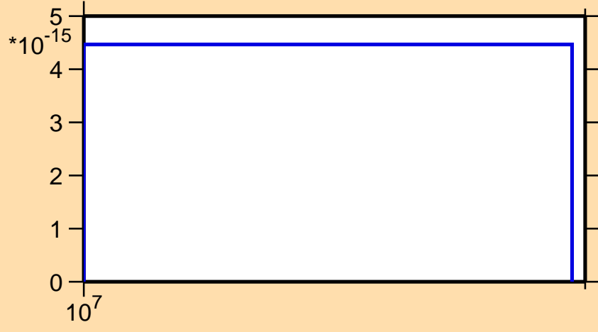
\sigma vs. E for ^{239}\text{Np} (mt 45)
