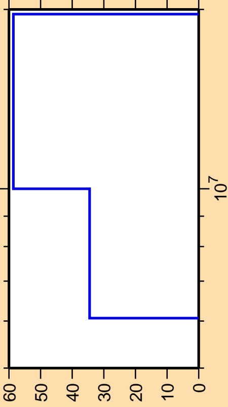
\Delta\sigma/\sigma vs. E for ^{239}\text{Np}(n,n\text{cont.})
