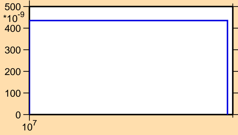
\sigma vs. E for ^{239}\text{Np}(n,3n\alpha)
