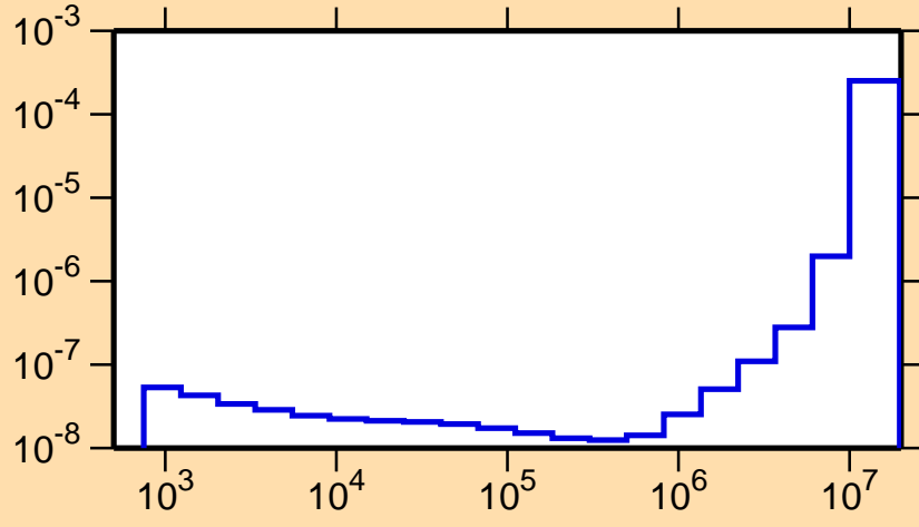
\sigma vs. E for ^{239}\text{Np}(n,\alpha)
