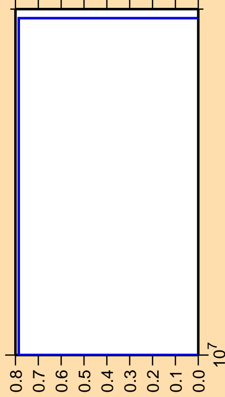
\Delta\sigma/\sigma vs. E for ^{239}\text{Np}(n,p\alpha)
