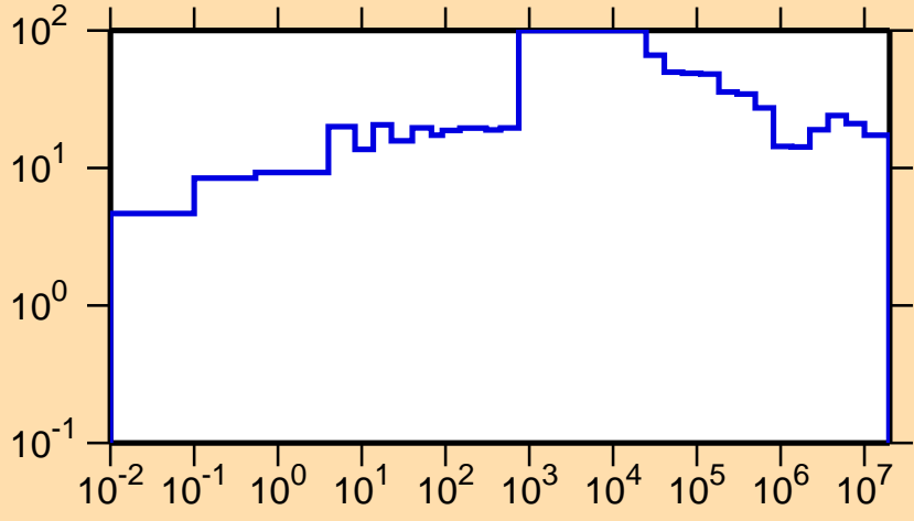
\Delta\sigma/\sigma vs. E for ^{239}\text{Np}(n,tot.)
