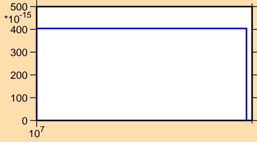
\sigma vs. E for ^{239}\text{Np}(n,p\alpha)
