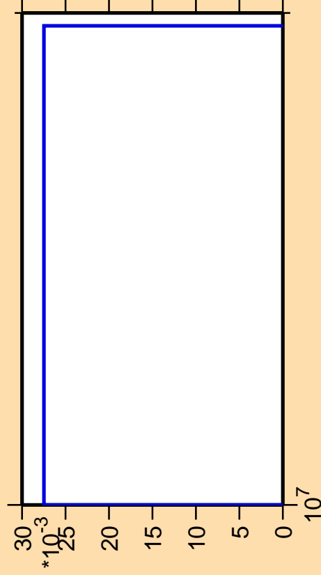
\Delta\sigma/\sigma vs. E for ^{239}\text{Np} (mt 45)
