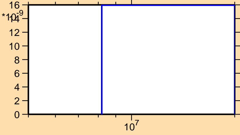
\sigma vs. E for ^{239}\text{Np}(n,nd)
