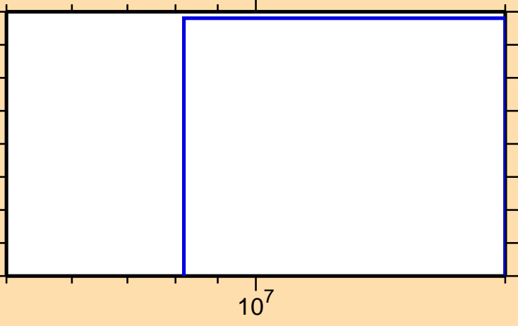
\sigma vs. E for ^{239}\text{Np}(n,t)
