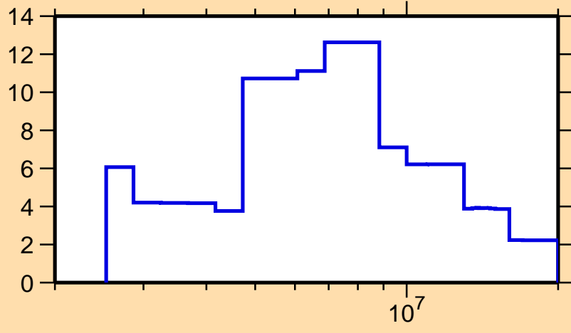
\Delta\sigma/\sigma vs. E for ^{240}\text{Np}(n,\text{tot.})
