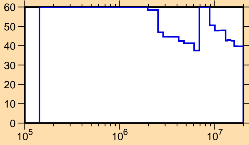
\Delta\sigma/\sigma vs. E for ^{240}\text{Np}(n,n\text{cont.})
