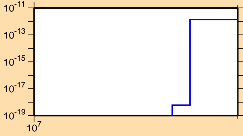
\sigma vs. E for ^{240}\text{Np} (mt 11)
