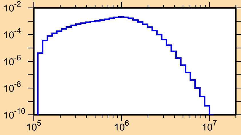
\sigma vs. E for ^{240}\text{Np}(n,n_1)
