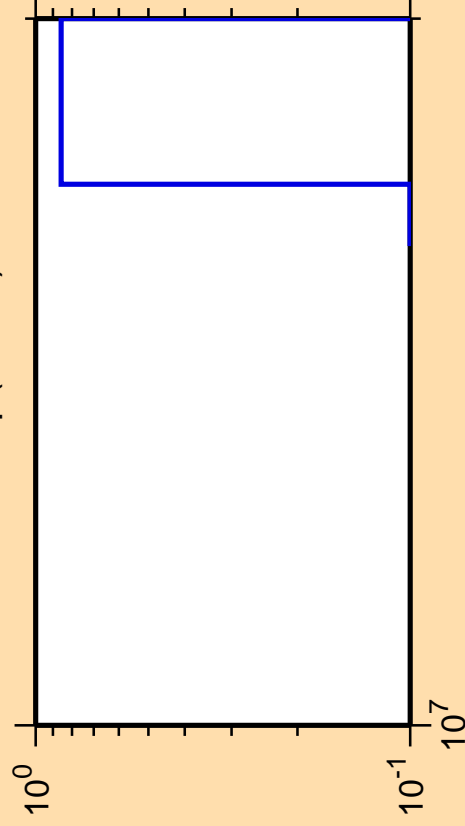
\Delta\sigma/\sigma vs. E for ^{240}\text{Np} (mt 11)
