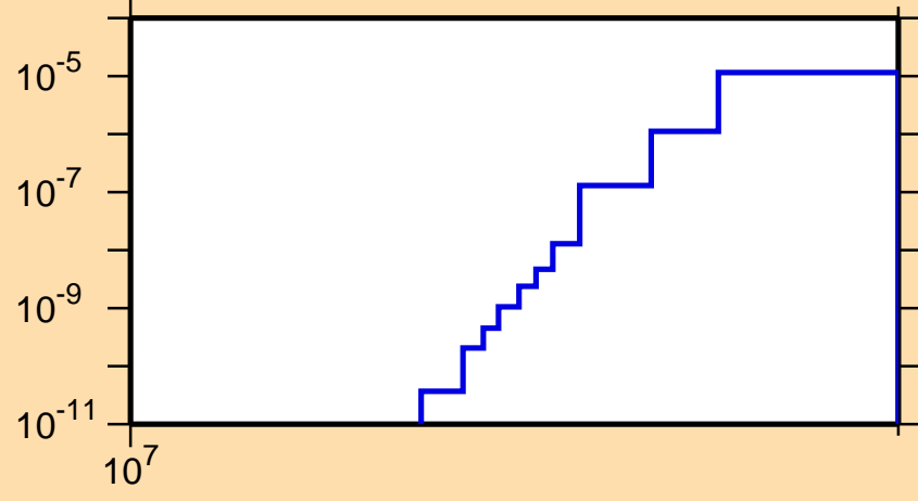
\sigma vs. E for ^{240}\text{Np}(n,\text{nd})
