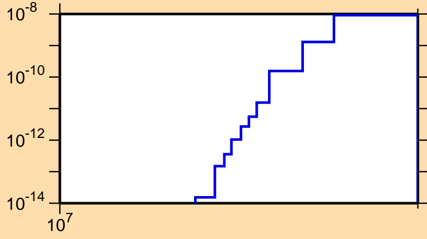
\sigma vs. E for ^{240}\text{Np}(n,3n\alpha)
