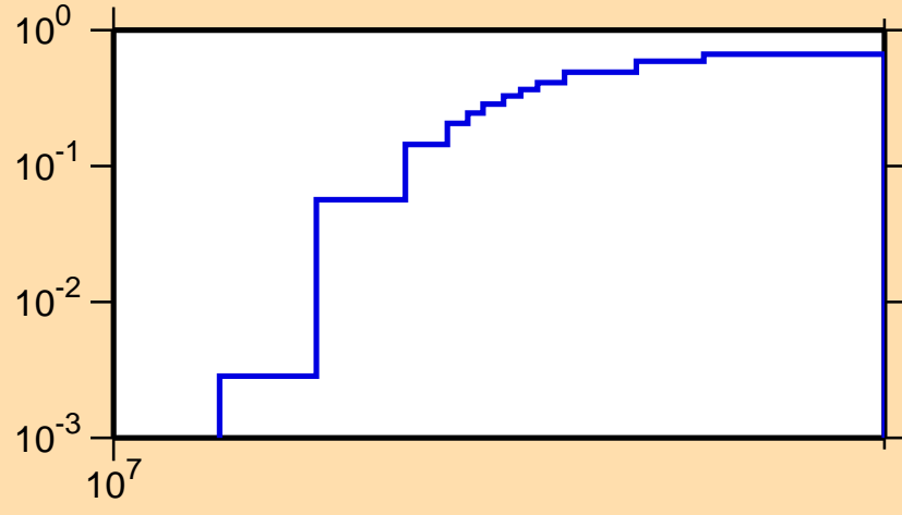
\sigma vs. E for ^{240}\text{Np}(n,3n)
