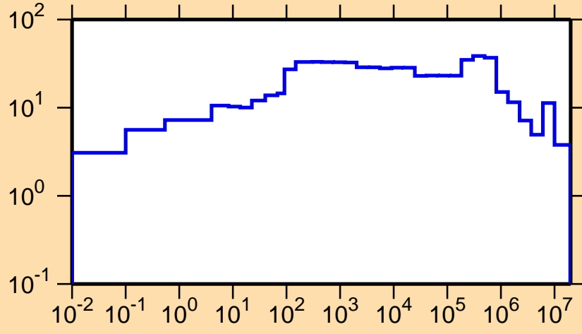
\Delta\sigma/\sigma vs. E for ^{240}\text{Np}(n,tot.)
