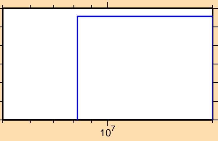
\sigma vs. E for ^{240}\text{Np}(n,np)
