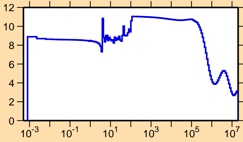
\sigma vs. E for ^{241}\text{Np}(n,\text{el.})
