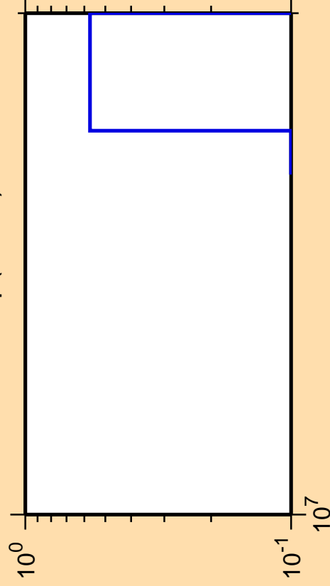
\Delta\sigma/\sigma vs. E for ^{241}\text{Np} (mt 42)
