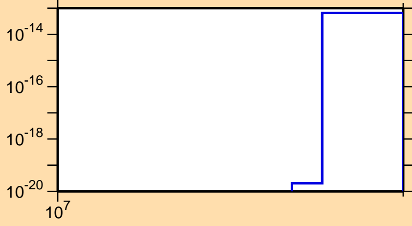
\sigma vs. E for ^{241}\text{Np} (mt 42)
