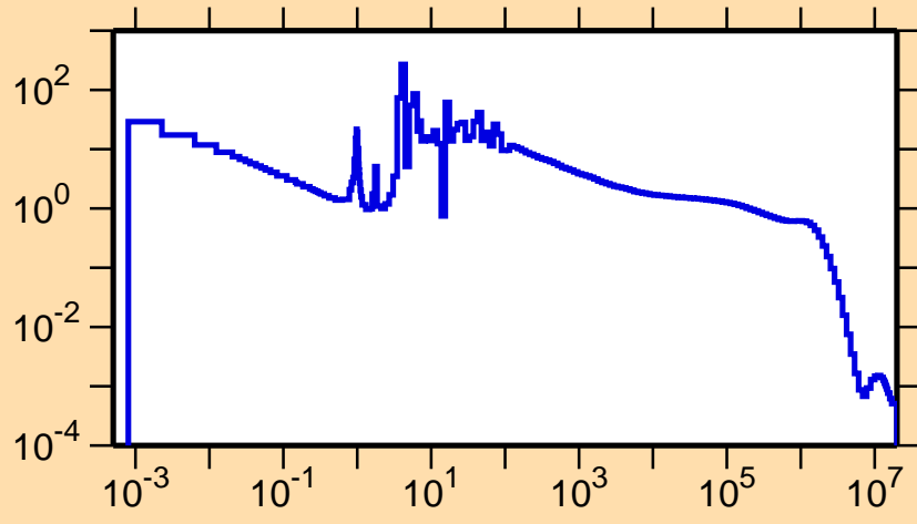
\sigma vs. E for ^{241}\text{Np}(n,\gamma)
