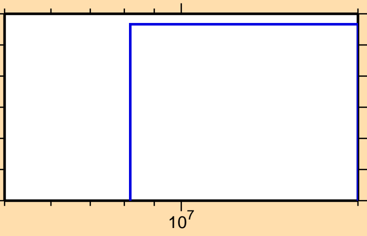
\sigma vs. E for ^{241}\text{Np}(n,\text{He}3)
