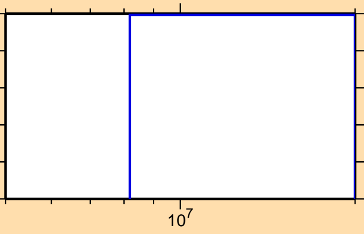
\sigma vs. E for ^{241}\text{Np}(n,2n\alpha)
