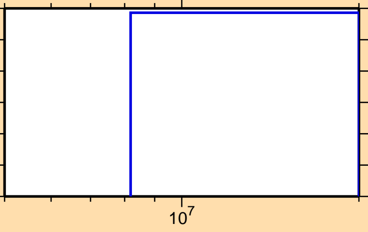
\sigma vs. E for ^{241}\text{Np}(n,\text{nd})
