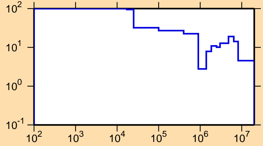
\Delta\sigma/\sigma vs. E for ^{241}\text{Np}(n,\text{tot.})
