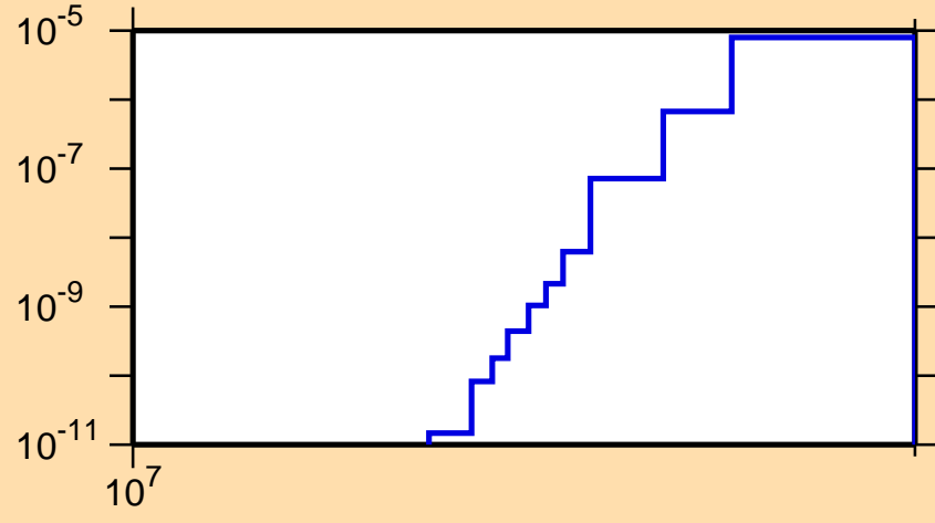
\sigma vs. E for ^{242}\text{Np}(n,nd)
