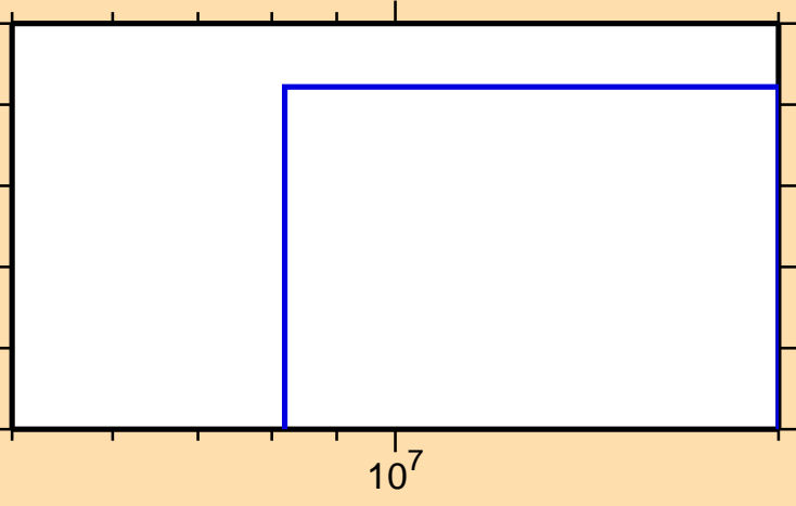
\sigma vs. E for ^{242}\text{Np}(n,np)
