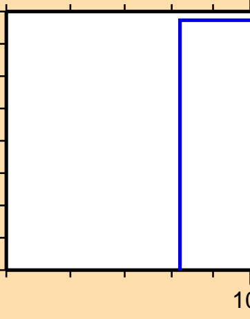
\sigma vs. E for ^{242}\text{Np}(n,\text{He3})
