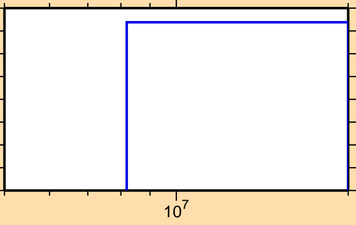
\sigma vs. E for ^{242}\text{Np}(n,d)
