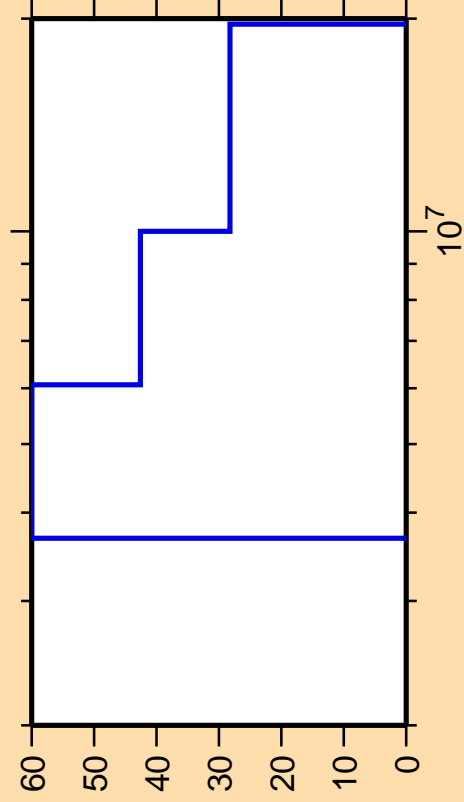
\Delta\sigma/\sigma vs. E for ^{242}\text{Np}(n,2n)
