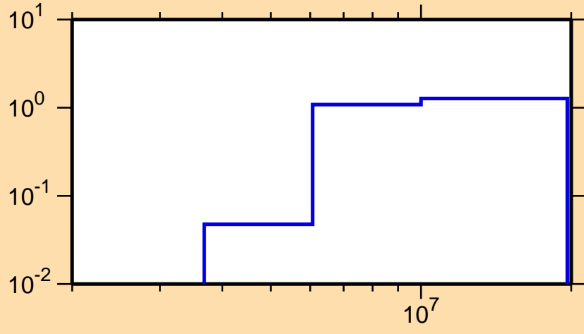
\sigma vs. E for ^{242}\text{Np}(n,2n)
