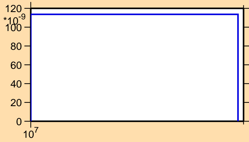
\sigma vs. E for ^{242}\text{Np}(n,nd)
