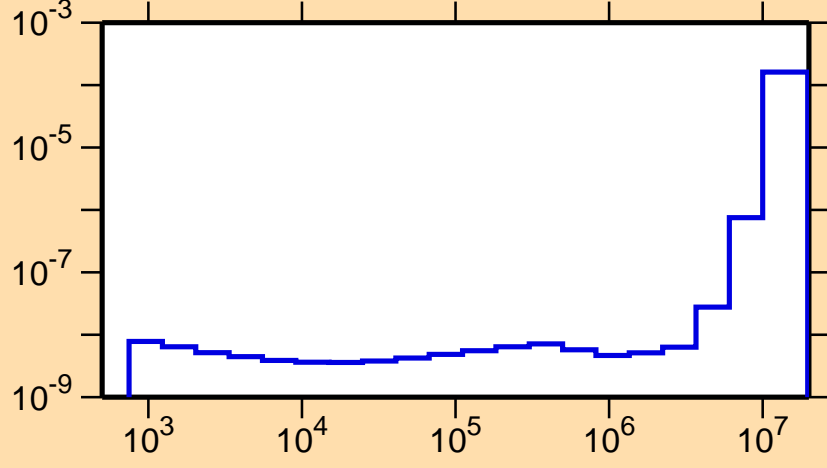
\sigma vs. E for ^{242}\text{Np}(n,\alpha)
