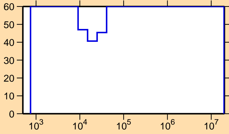
\Delta\sigma/\sigma vs. E for ^{242}\text{Np}(n,\gamma)
