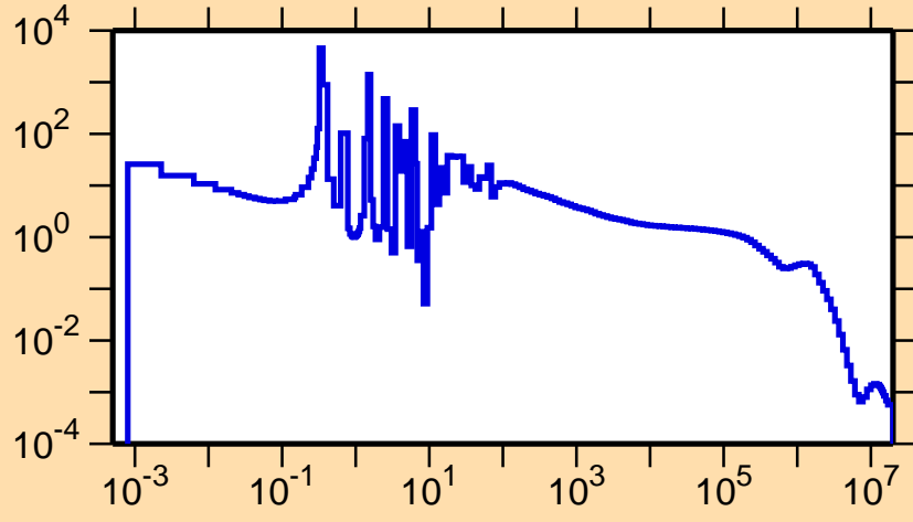
\sigma vs. E for ^{243}\text{Np}(n,\gamma)
