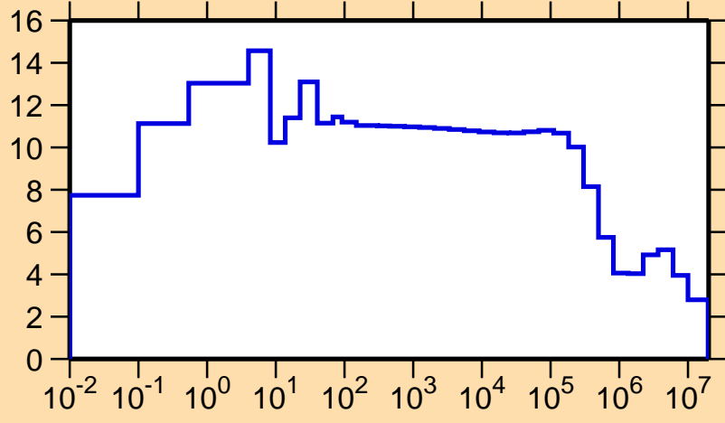
\sigma vs. E for ^{243}\text{Np}(n,\text{el.})
