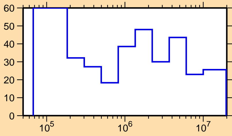
\Delta\sigma/\sigma vs. E for ^{243}\text{Np}(n,n_1)
