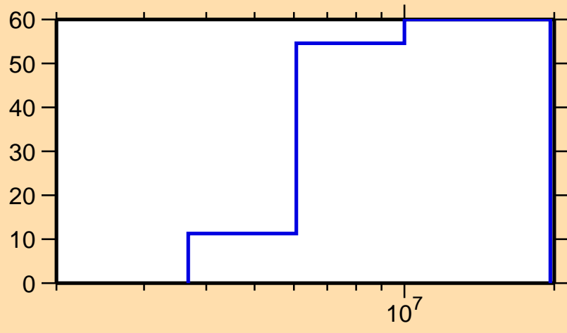
\Delta\sigma/\sigma vs. E for ^{243}\text{Np}(n,p)
