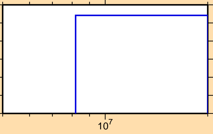
\sigma vs. E for ^{243}\text{Np}(n,t)
