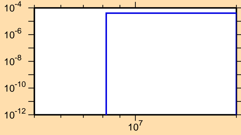
\sigma vs. E for ^{243}\text{Np}(n,d)
