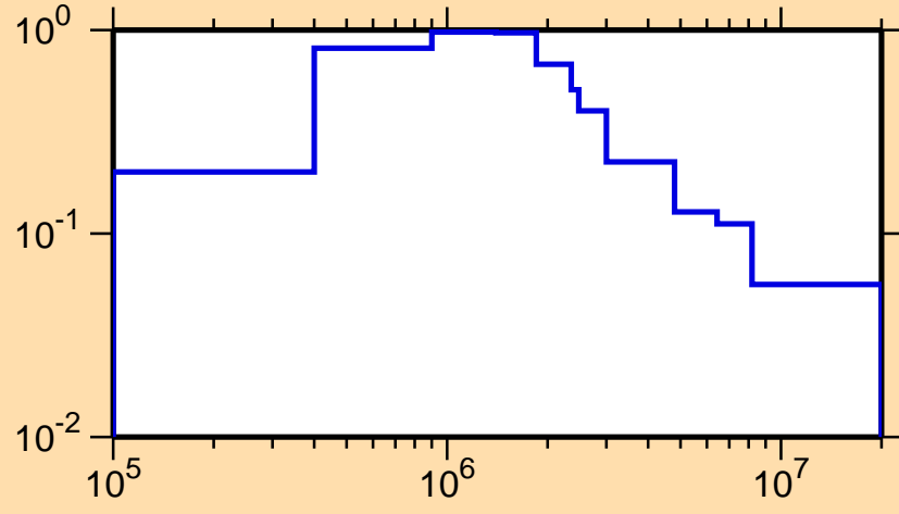
\sigma vs. E for ^{243}\text{Np}(n,n_3)
