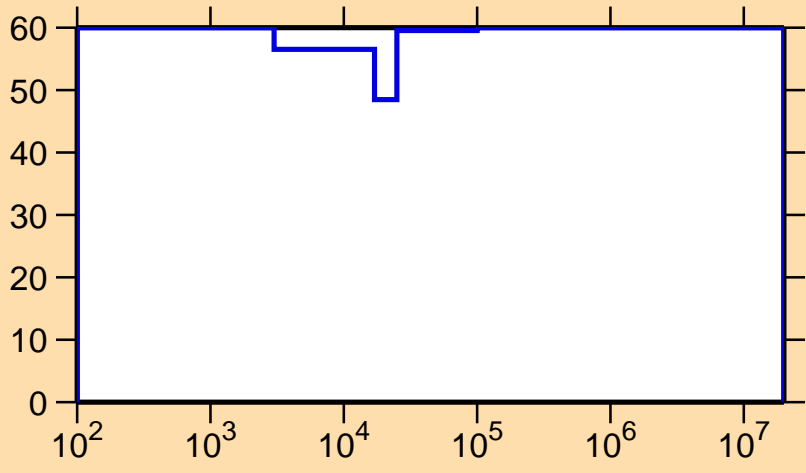
\Delta\sigma/\sigma vs. E for ^{243}\text{Np}(n,\gamma)
