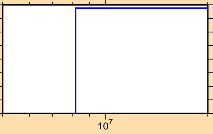
\sigma vs. E for ^{243}\text{Np}(\text{mt } 11)
