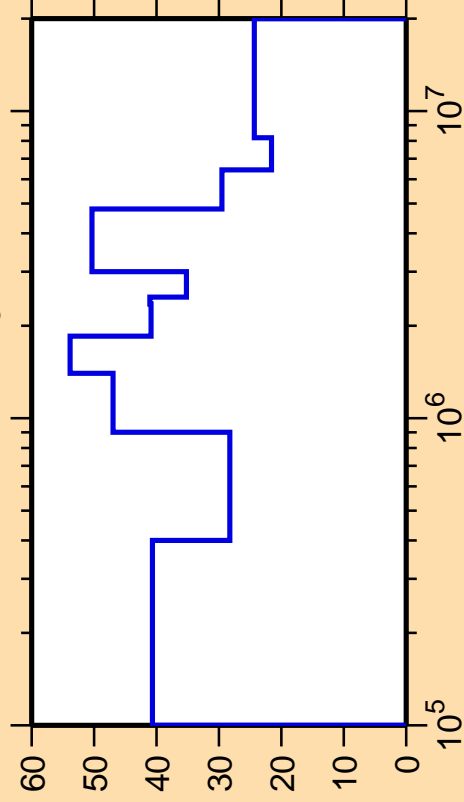
\Delta\sigma/\sigma vs. E for ^{243}\text{Np}(n,n_3)
