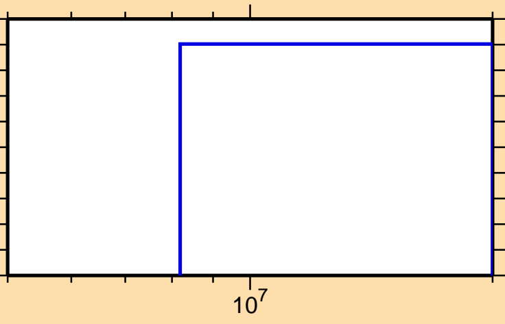
\sigma vs. E for ^{243}\text{Np}(n,\text{nd})
