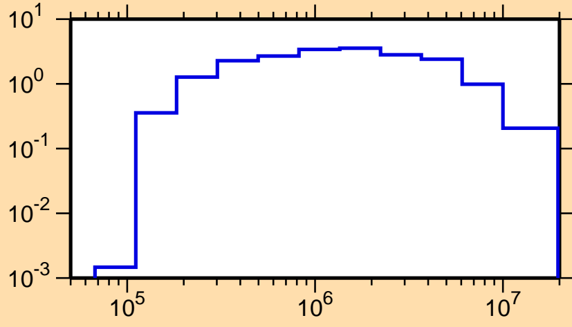
\sigma vs. E for ^{244}\text{Np}(n,\text{inel.})
