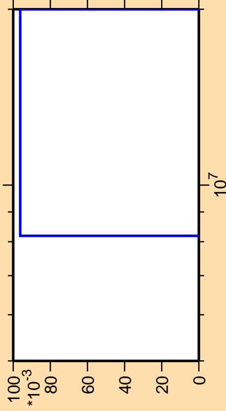
\Delta\sigma/\sigma vs. E for ^{244}\text{Np}(\text{mt } 11)
