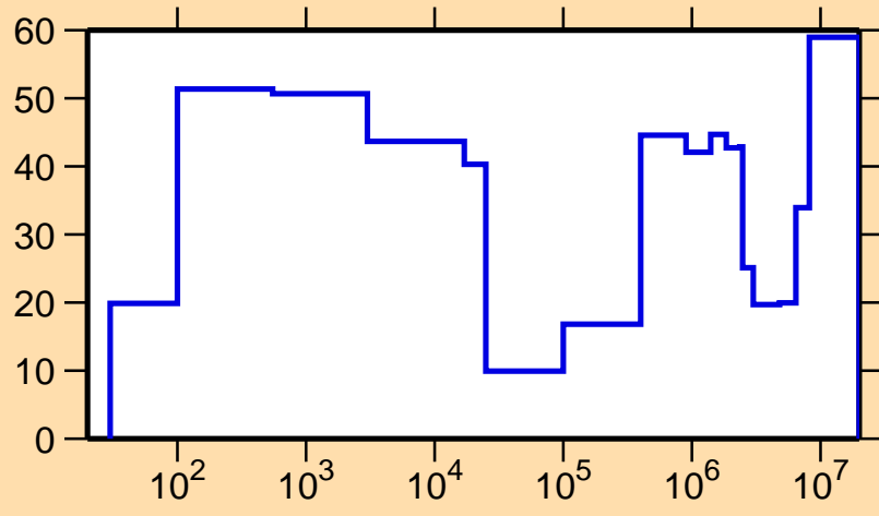
\Delta\sigma/\sigma vs. E for ^{244}\text{Np}(n,\text{el.})
