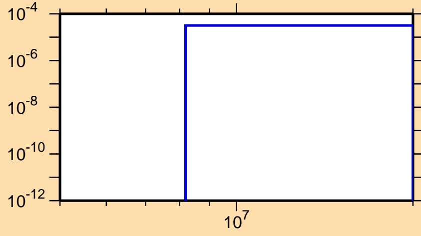
\sigma vs. E for ^{244}\text{Np}(n,t)
