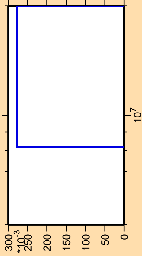
\Delta\sigma/\sigma vs. E for ^{244}\text{Np}(n,p\alpha)
