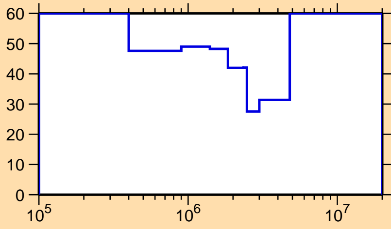
\Delta\sigma/\sigma vs. E for ^{244}\text{Np}(n,\text{inel.})
