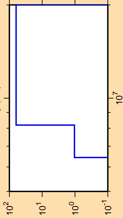
\Delta\sigma/\sigma vs. E for ^{244}\text{Np}(n,t)
