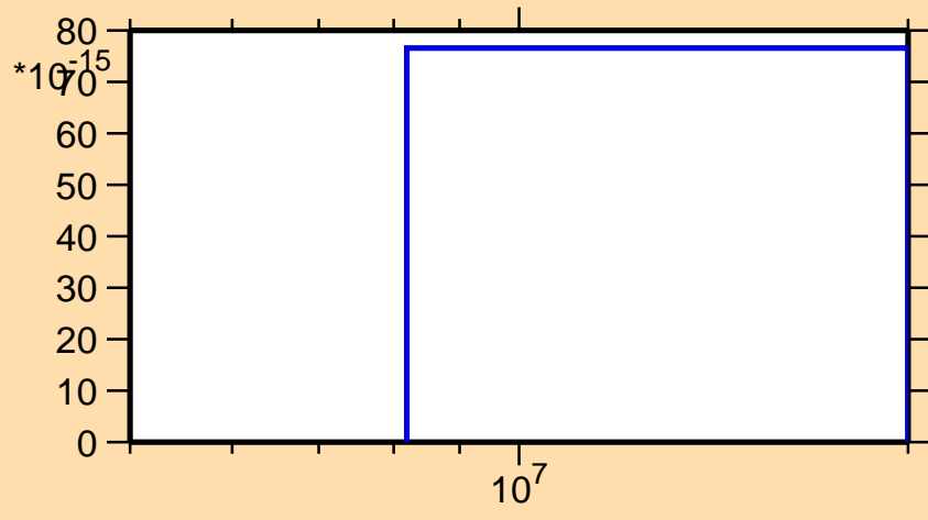
\sigma vs. E for ^{244}\text{Np}(n,p\alpha)
