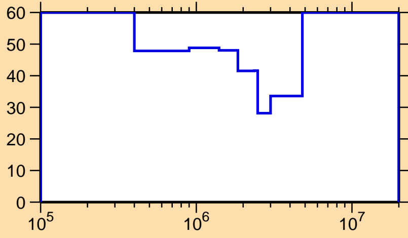
\Delta\sigma/\sigma vs. E for ^{244}\text{Np}(n,n\text{cont.})
