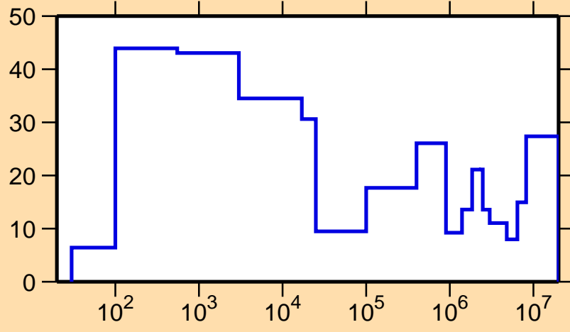
\Delta\sigma/\sigma vs. E for ^{244}\text{Np}(n,\text{tot.})
