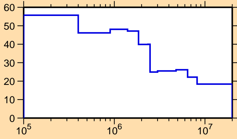
\Delta\sigma/\sigma vs. E for ^{244}\text{Np}(n,\text{nonel.})
