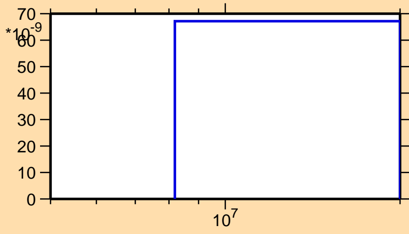
\sigma vs. E for ^{244}\text{Np}(n,\text{nd})
