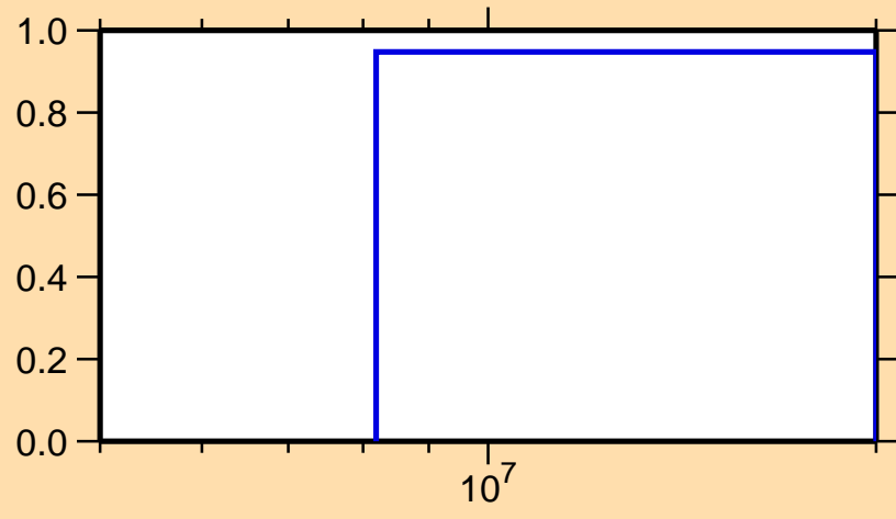
\sigma vs. E for ^{244}\text{Np}(n,3n)
