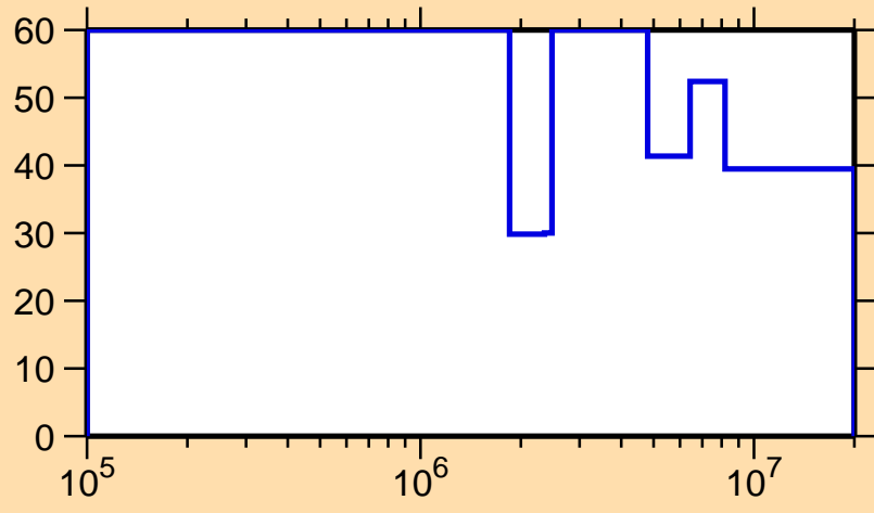
\Delta\sigma/\sigma vs. E for ^{244}\text{Np}(n,n_1)
