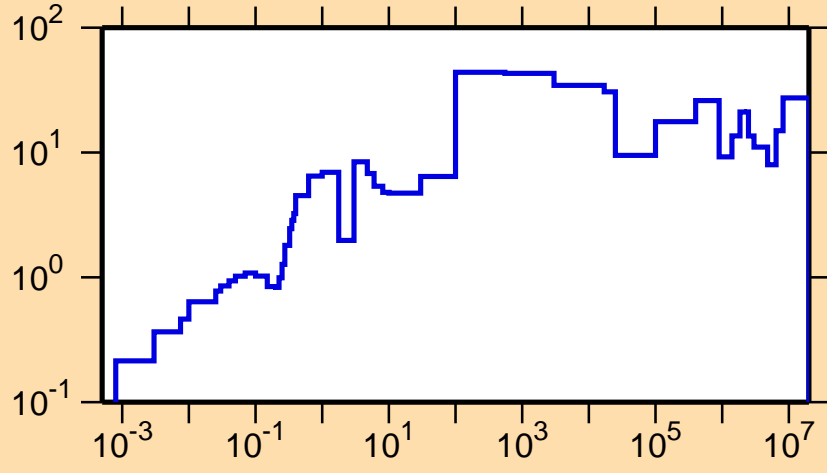
\Delta\sigma/\sigma vs. E for ^{244}\text{Np}(n,tot.)
