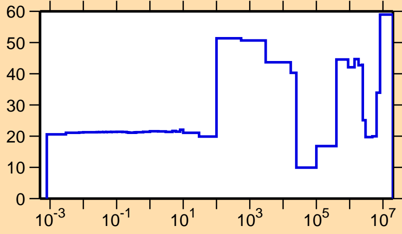
\Delta\sigma/\sigma vs. E for ^{244}\text{Np}(n,el.)
