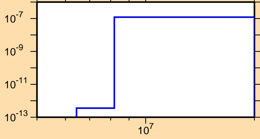
\sigma vs. E for ^{244}\text{Np}(n,2n\alpha)
