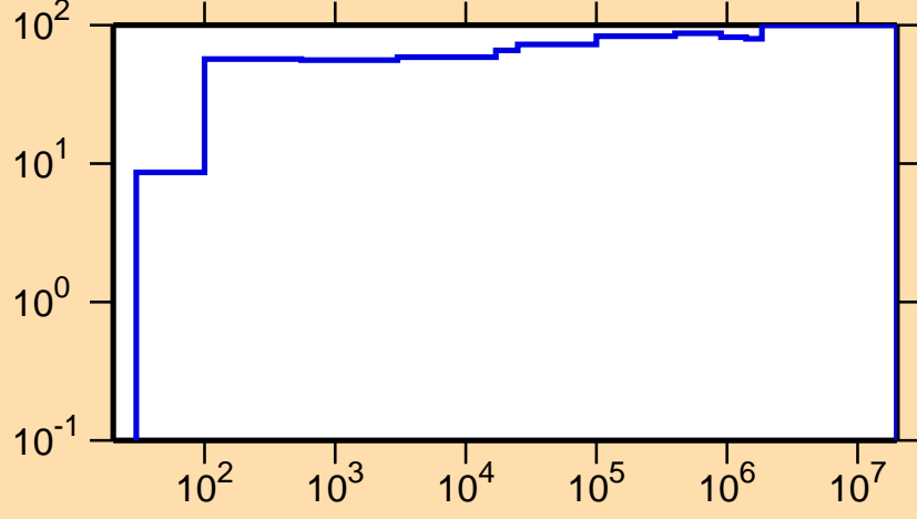
\Delta\sigma/\sigma vs. E for ^{244}\text{Np}(n,\gamma)
