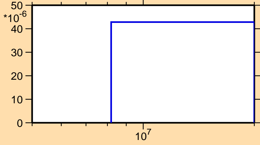
\sigma vs. E for ^{244}\text{Np}(n,d)
