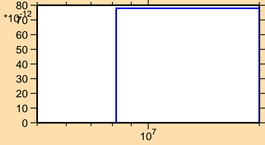
\sigma vs. E for ^{244}\text{Np}(n,3n\alpha)
