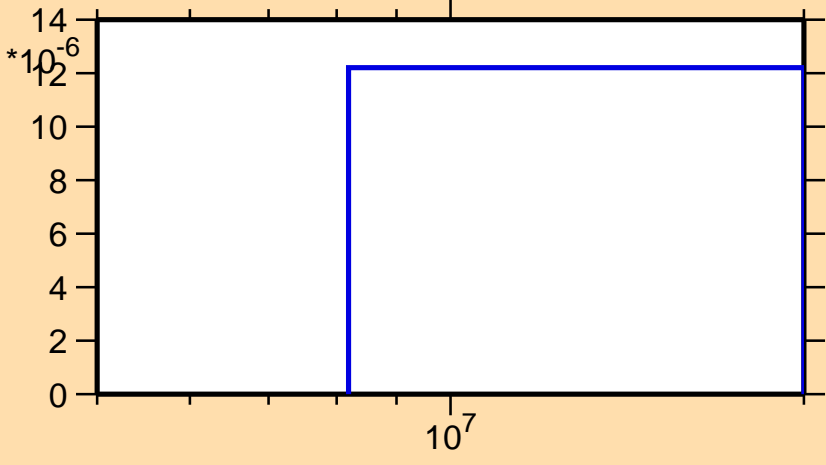
\sigma vs. E for ^{244}\text{Np}(n,np)
