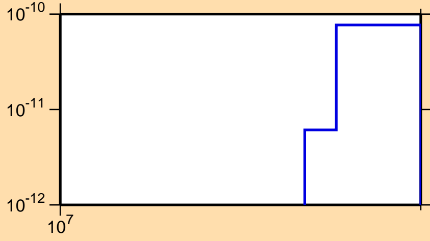
\sigma vs. E for ^{245}\text{Np}(\text{mt117})
