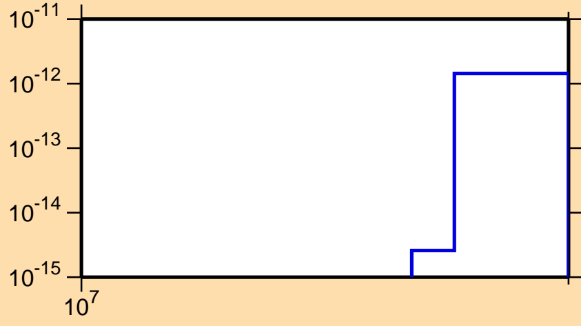
\sigma vs. E for ^{245}\text{Np}(\text{mt } 11)
