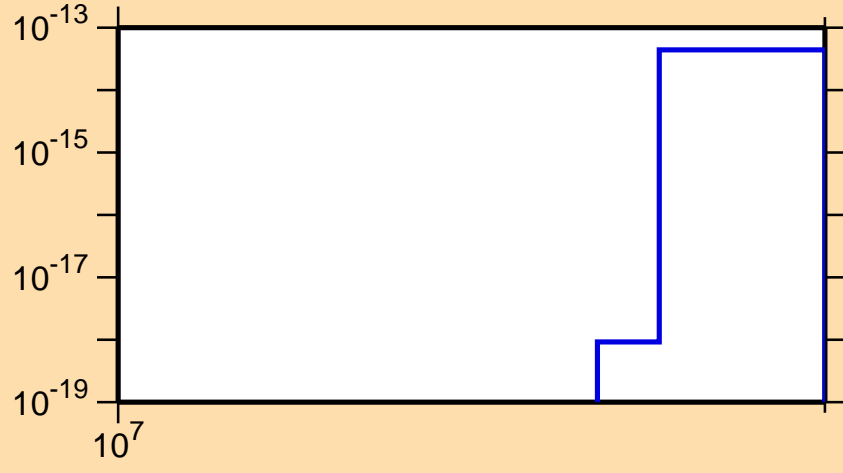
\sigma vs. E for ^{245}\text{Np}(n,\text{He3})
