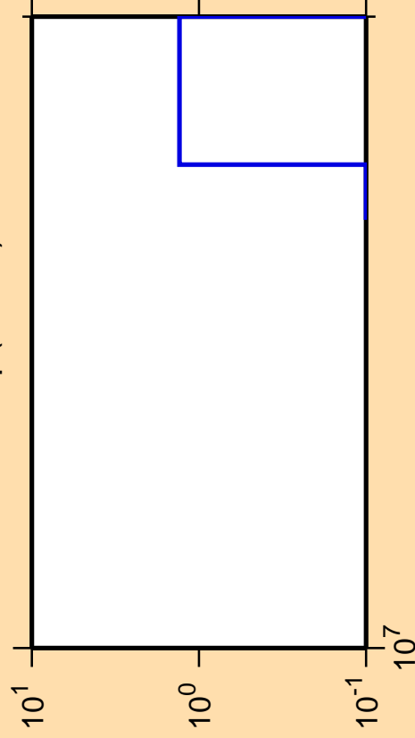
\Delta\sigma/\sigma vs. E for ^{245}\text{Np}(\text{mt } 11)
