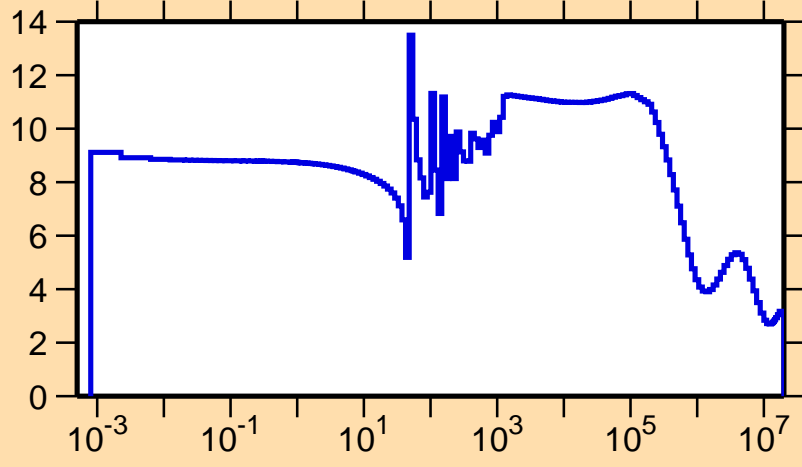
\sigma vs. E for ^{245}\text{Np}(n,\text{el.})
