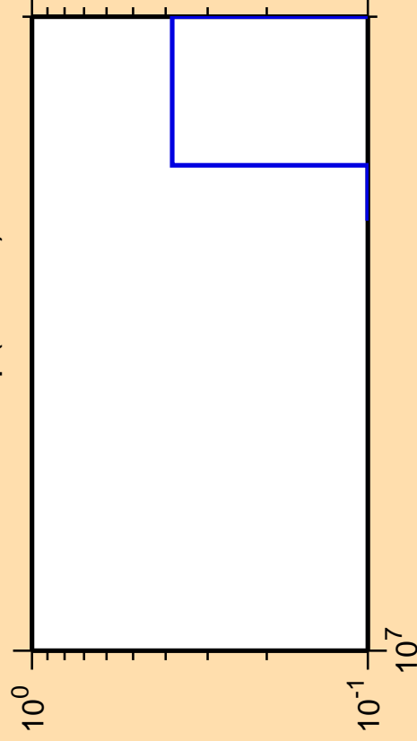
\Delta\sigma/\sigma vs. E for ^{245}\text{Np}(n,\text{He3})
