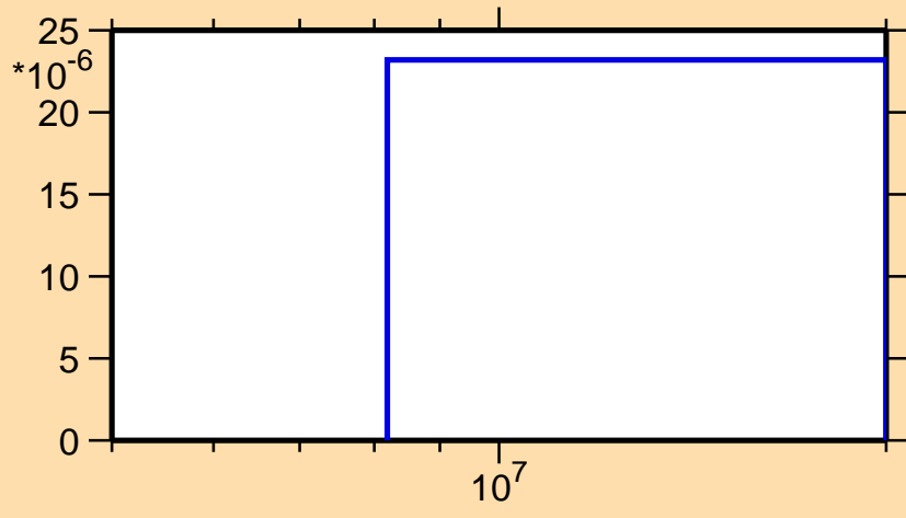
\sigma vs. E for ^{245}\text{Np}(n,np)
