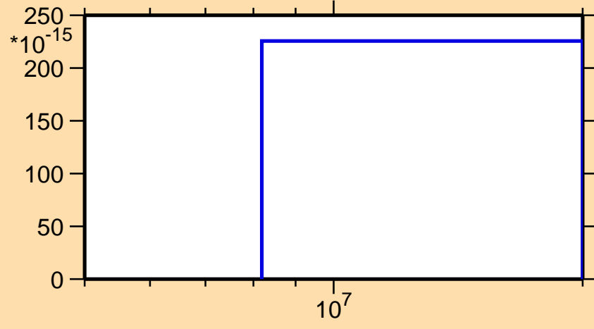
\sigma vs. E for ^{245}\text{Np} (mt 45)
