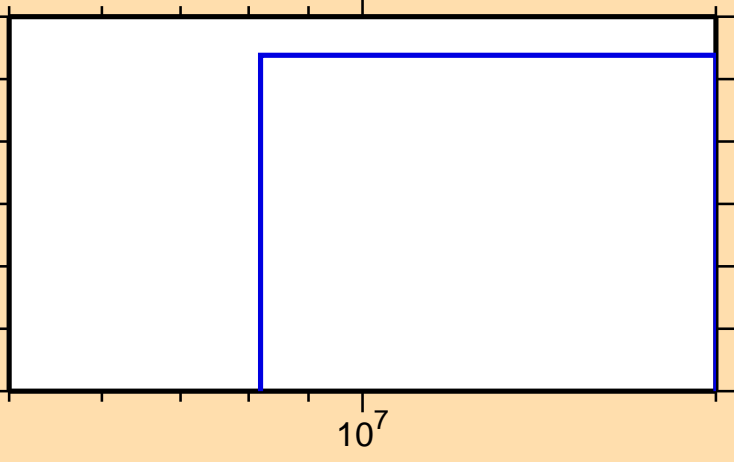
\sigma vs. E for ^{245}\text{Np}(n,2np)
