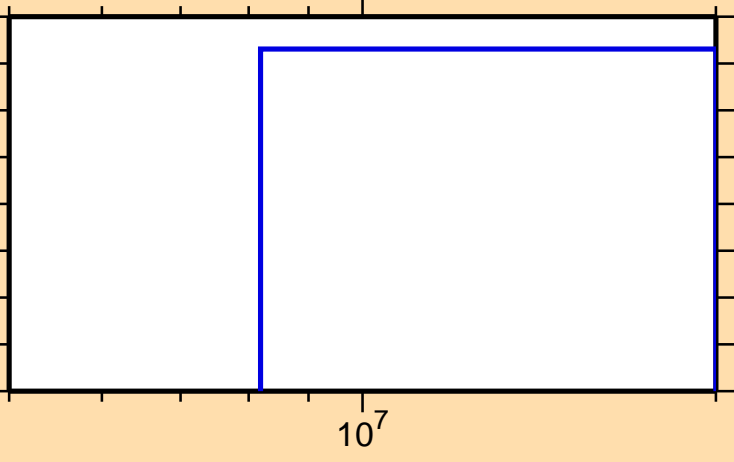
\sigma vs. E for ^{245}\text{Np}(n,d)
