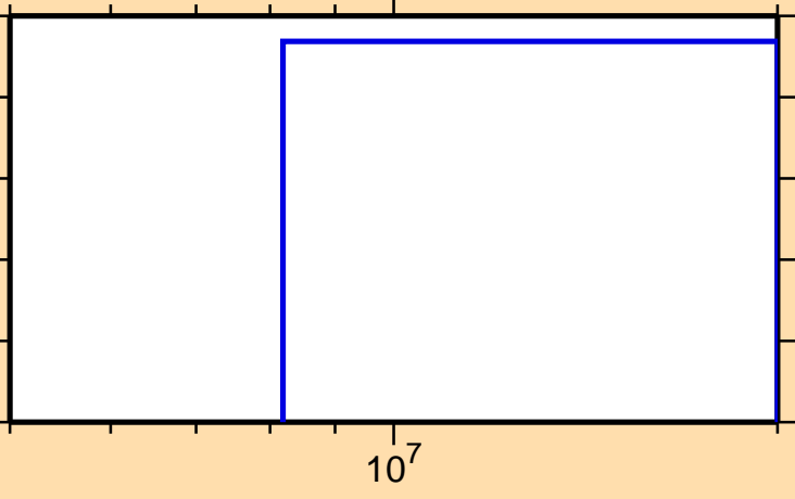
\sigma vs. E for ^{245}\text{Np}(n,nt)
