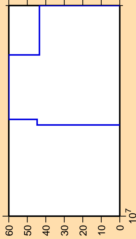
\Delta\sigma/\sigma vs. E for ^{14}\text{O} (mt117)
