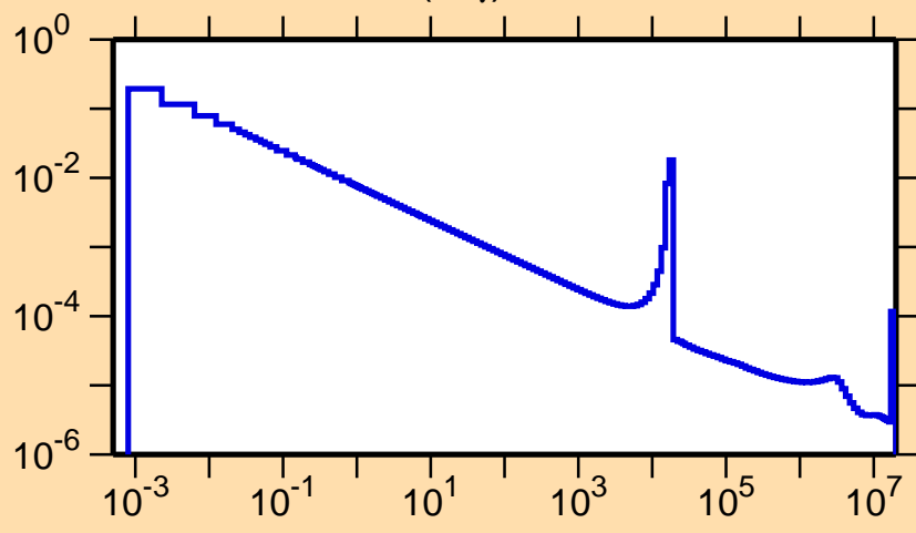
\sigma vs. E for ^{14}\text{O}(n,\gamma)
