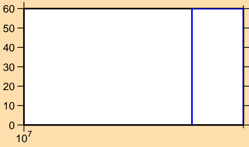
\Delta\sigma/\sigma vs. E for ^{14}\text{O}(n,ncont.)
