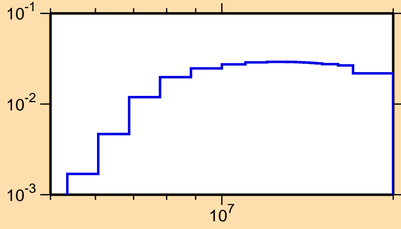
\sigma vs. E for ^{14}\text{O}(n,\text{inel.})
