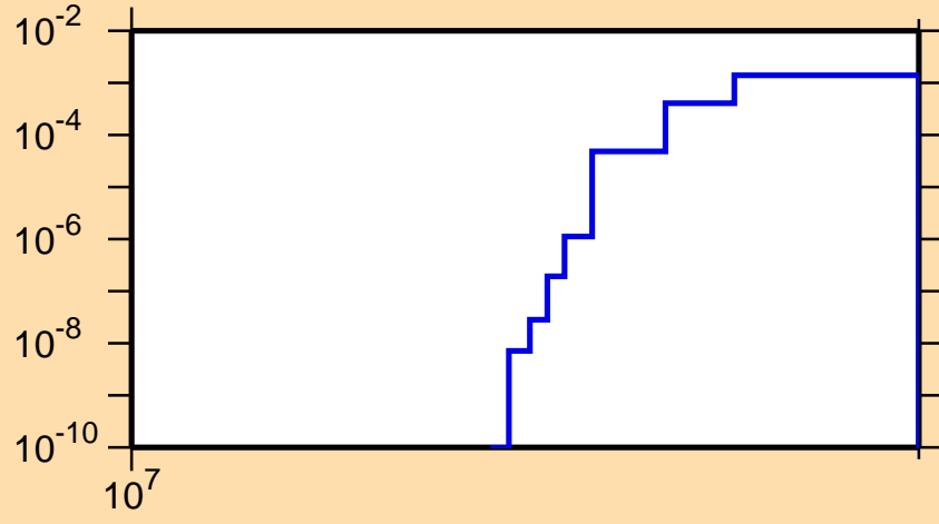
\sigma vs. E for ^{14}\text{O} (mt117)
