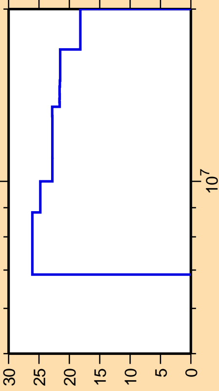
\Delta\sigma/\sigma vs. E for ^{14}\text{O}(n,n_4)
