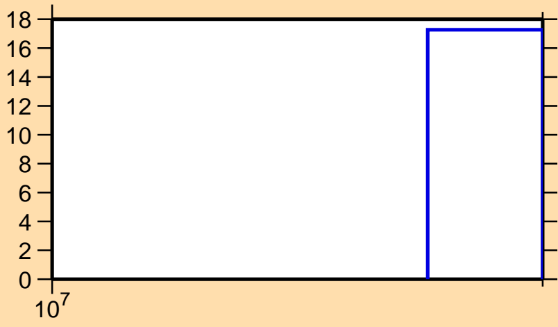
\Delta\sigma/\sigma vs. E for ^{14}\text{O}(n,n_1)
