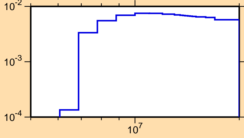
\sigma vs. E for ^{14}\text{O}(n,n_3)
