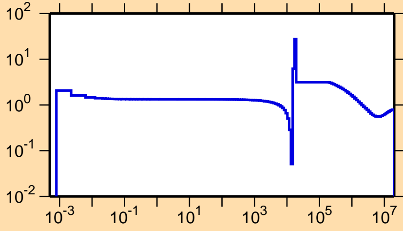
\sigma vs. E for ^{14}\text{O}(n,\text{el.})
