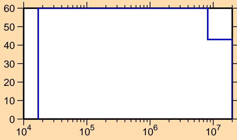
\Delta\sigma/\sigma vs. E for ^{14}\text{O}(n,\gamma)
