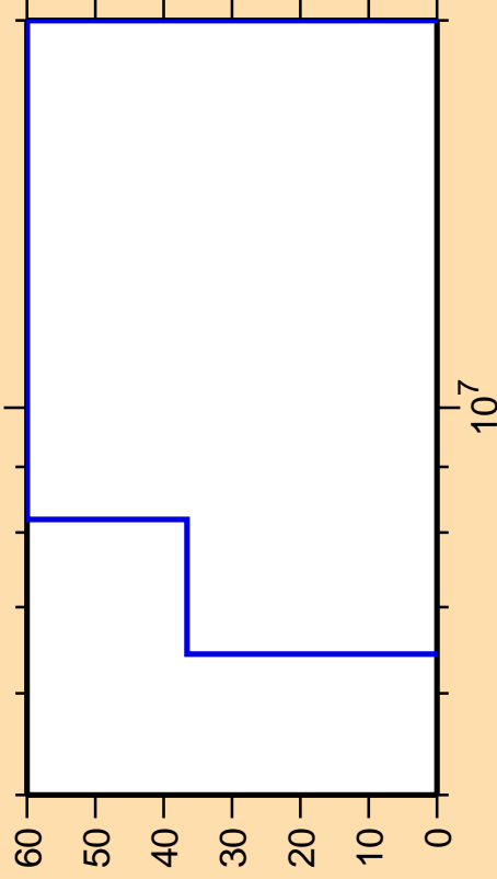
\Delta\sigma/\sigma vs. E for ^{15}\text{O}(n,n_3)
