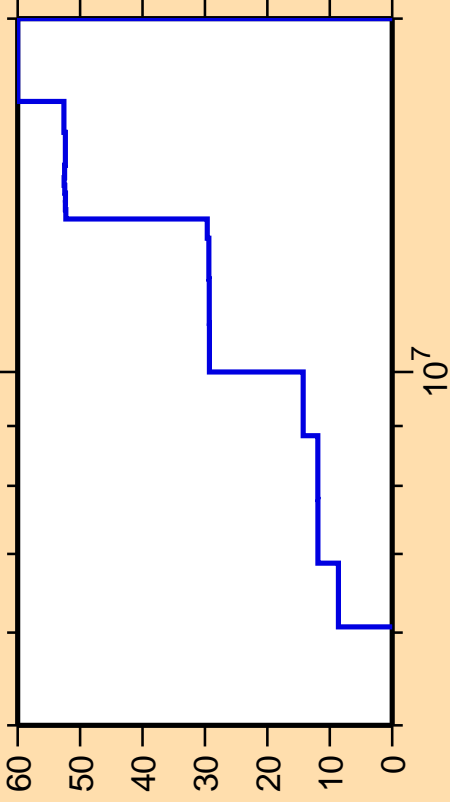
\Delta\sigma/\sigma vs. E for ^{17}\text{O}(n,n_1)
