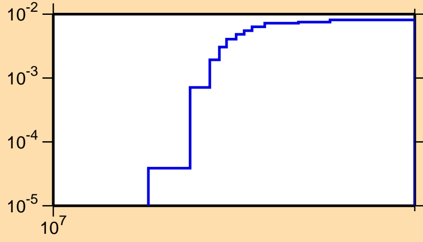
\sigma vs. E for ^{17}\text{O}(n,d)
