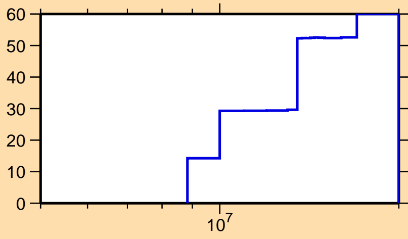
\Delta\sigma/\sigma vs. E for ^{17}\text{O}(n,n_1)
