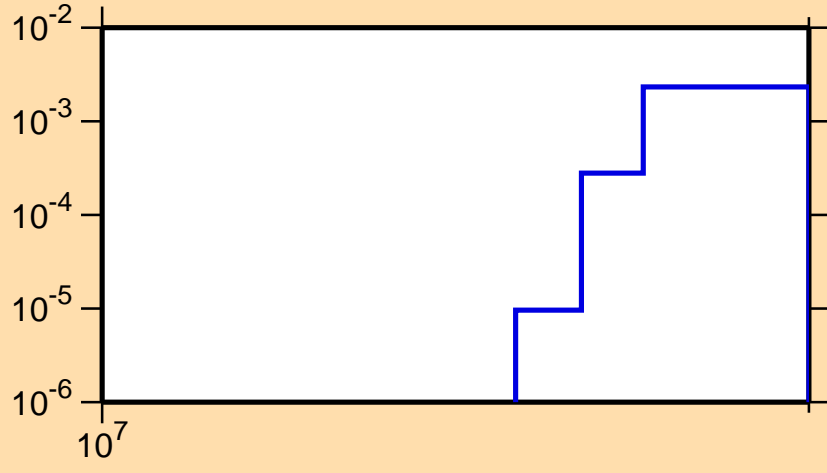
\sigma vs. E for ^{17}\text{O}(n,\text{nd})
