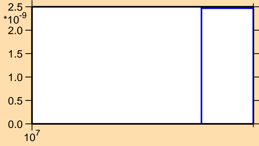
\sigma vs. E for ^{17}\text{O}(n,\text{He}3)
