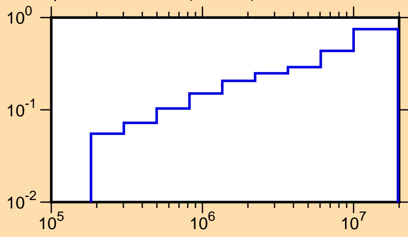
\mu vs. E for ^{17}\text{O}(\text{mt251})
