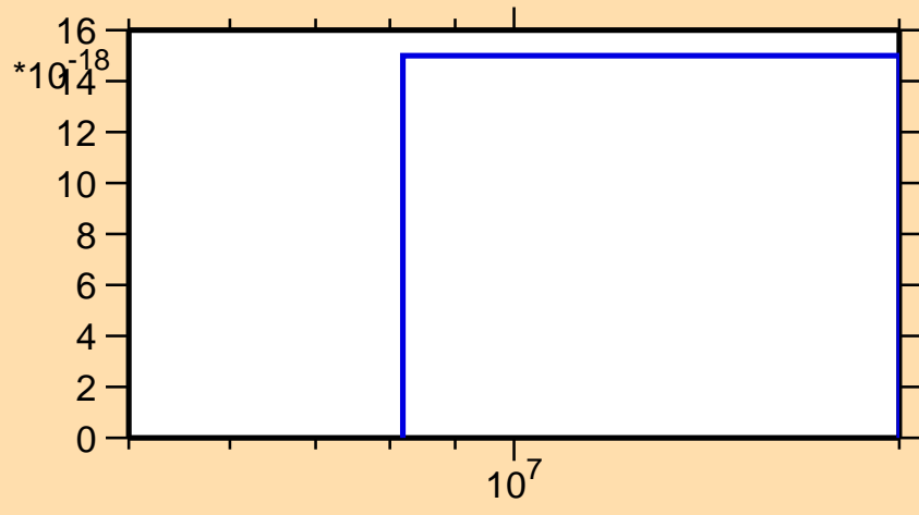
\sigma vs. E for ^{17}\text{O}(n,nt)
