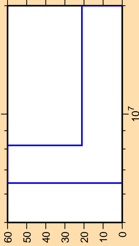
\Delta\sigma/\sigma vs. E for ^{17}\text{O}(n,2n)
