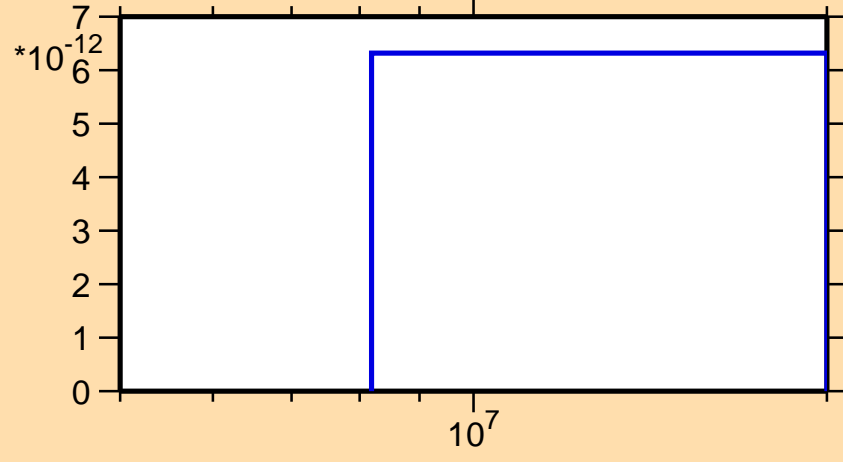
\sigma vs. E for ^{17}\text{O}(n,\text{pt})
