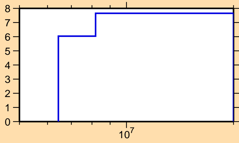
\Delta\sigma/\sigma vs. E for ^{17}\text{O}(n,\text{el.})
