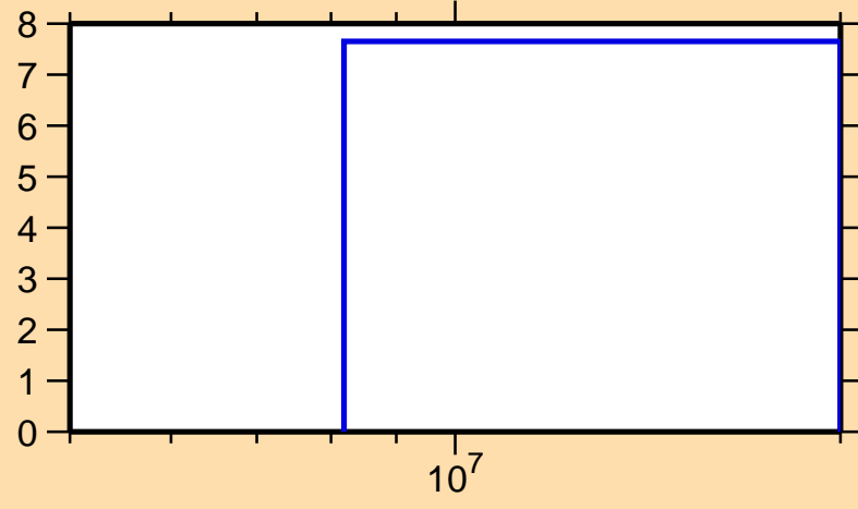
\Delta\sigma/\sigma vs. E for ^{17}\text{O}(n,el.)
