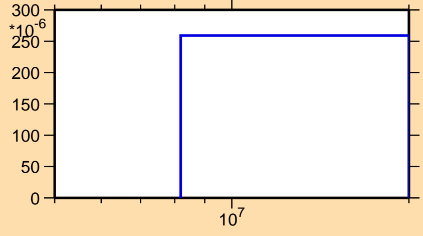
\sigma vs. E for ^{18}\text{O}(n,p)
