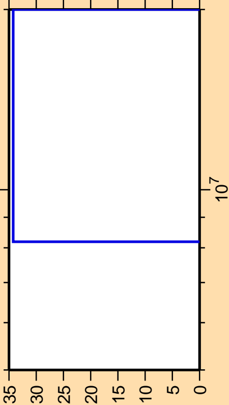
\Delta\sigma/\sigma vs. E for ^{18}\text{O}(n,p)
