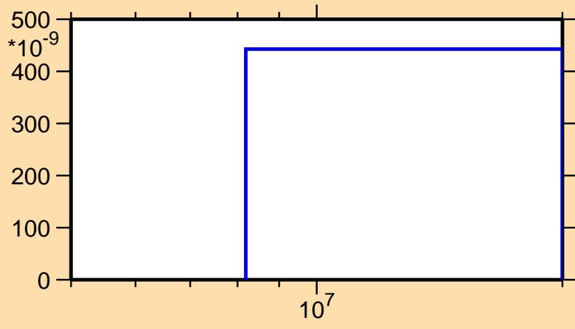
\sigma vs. E for ^{18}\text{O}(n,nt)
