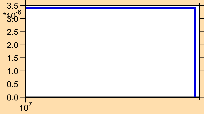
\sigma vs. E for ^{19}\text{O}(n,d)
