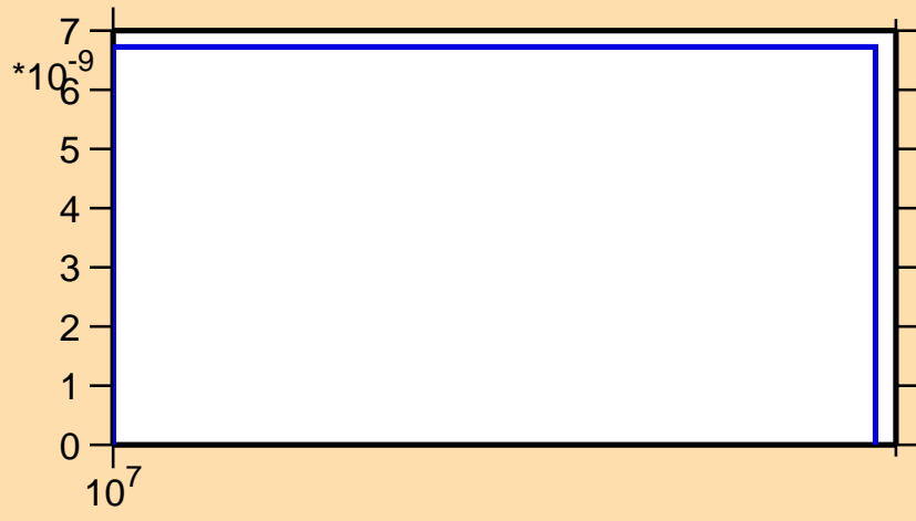
\sigma vs. E for ^{19}\text{O}(n,\text{nd})
