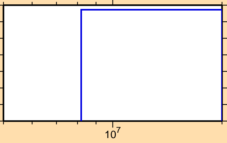
\sigma vs. E for ^{19}\text{O}(n,2n\alpha)
