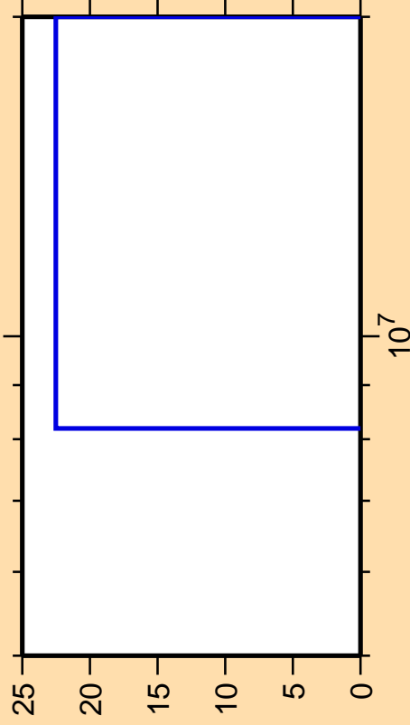
\Delta\sigma/\sigma vs. E for ^{19}\text{O}(n,p)
