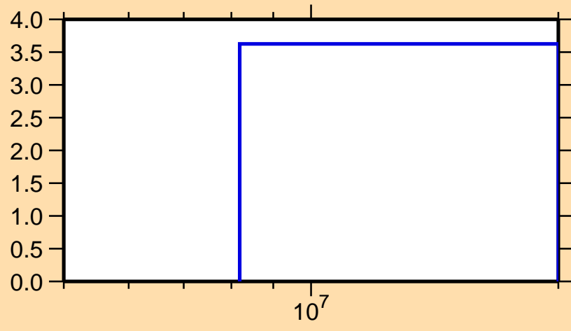
\Delta\sigma/\sigma vs. E for ^{19}\text{O}(n,el.)
