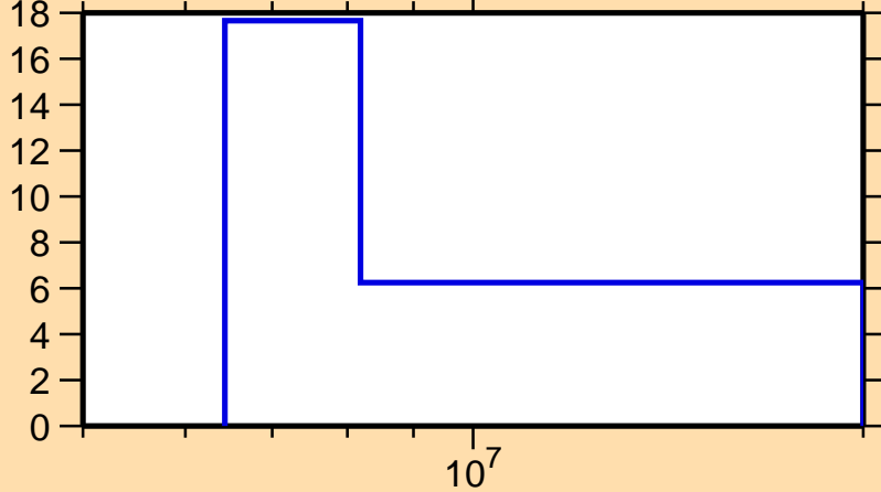
\Delta\sigma/\sigma vs. E for ^{19}\text{O}(n,2n)
