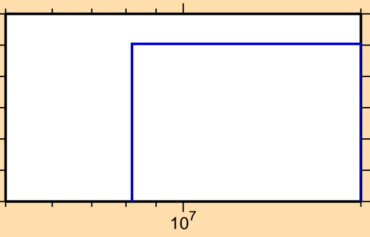
\sigma vs. E for ^{19}\text{O}(n,\text{nd})
