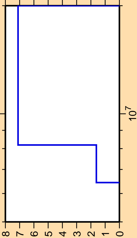
\Delta\sigma/\sigma vs. E for ^{19}\text{O}(n,n_1)
