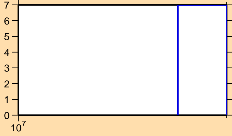
\Delta\sigma/\sigma vs. E for ^{20}\text{O}(n,el.)
