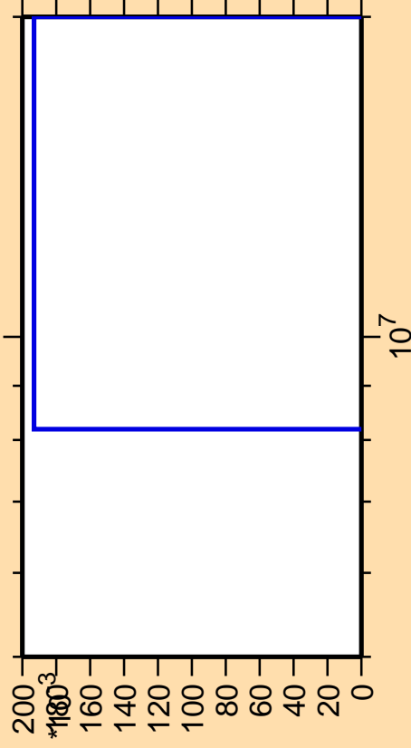
\Delta\sigma/\sigma vs. E for ^{20}\text{O}(n,nt)
