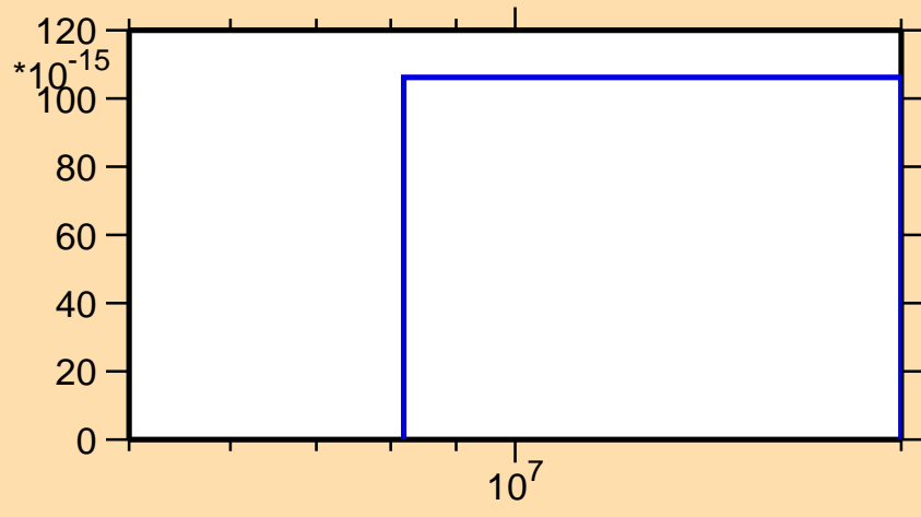
\sigma vs. E for ^{20}\text{O}(n,nt)
