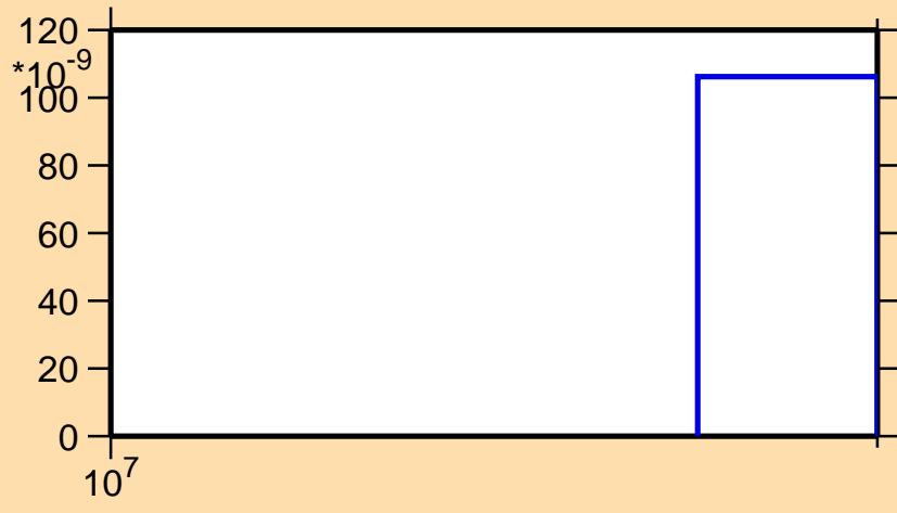
\sigma vs. E for ^{21}\text{O}(n,2n\alpha)
