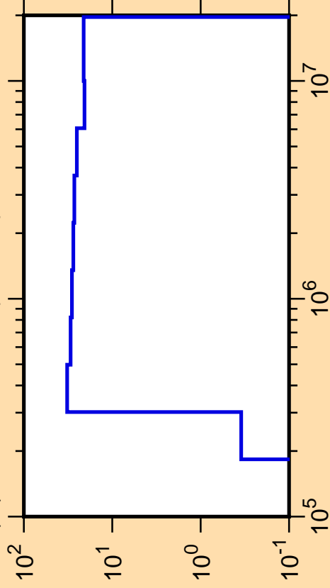
\Delta\mu/\mu vs. E for ^{21}\text{O}(\text{mt251})
