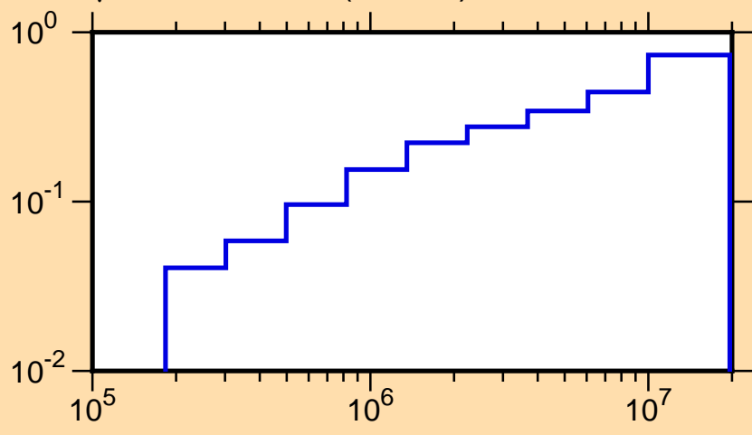
\mu vs. E for ^{21}\text{O}(\text{mt251})
