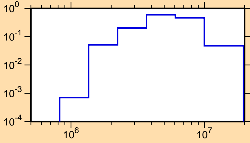
\sigma vs. E for ^{21}\text{O}(n,\text{inel.})
