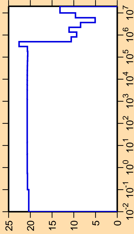
\Delta\sigma/\sigma vs. E for ^{21}\text{O}(n,\text{el.})
