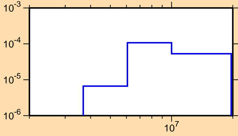
\sigma vs. E for ^{21}\text{O}(n,n\text{cont.})
