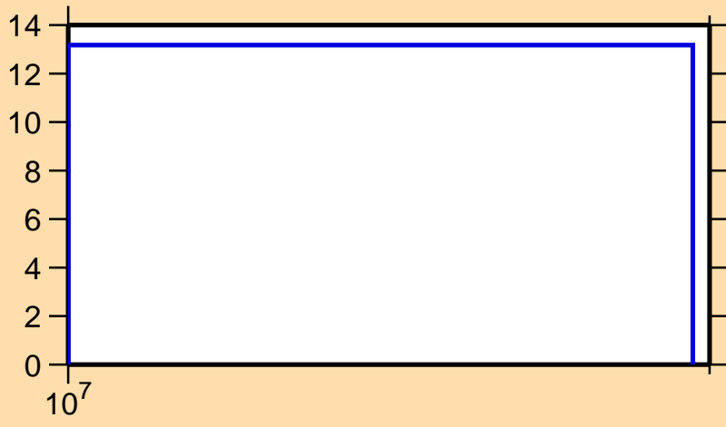
\Delta\sigma/\sigma vs. E for ^{21}\text{O}(n,el.)
