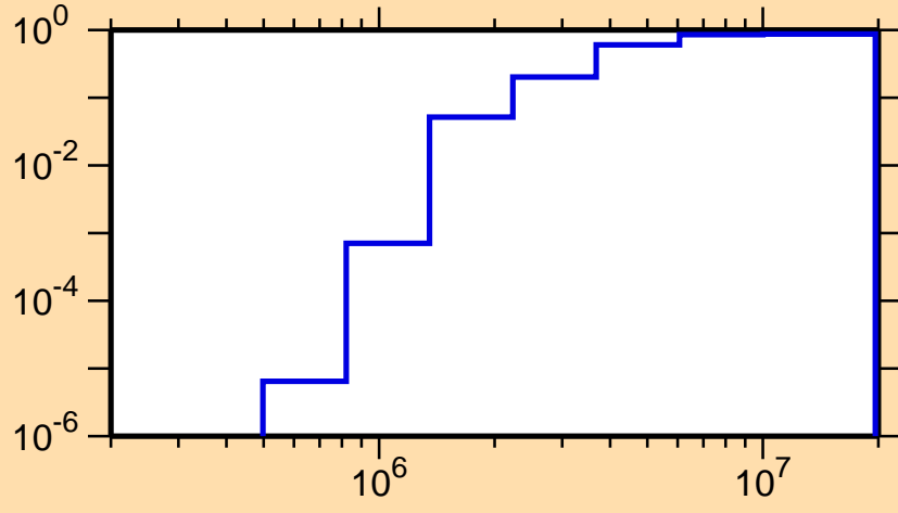
\sigma vs. E for ^{21}\text{O}(n,\text{nonel.})
