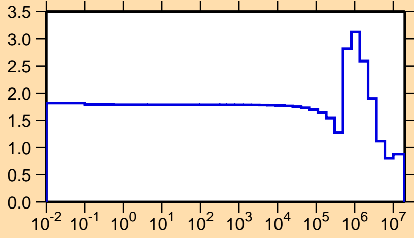
\sigma vs. E for ^{21}\text{O}(n,\text{el.})
