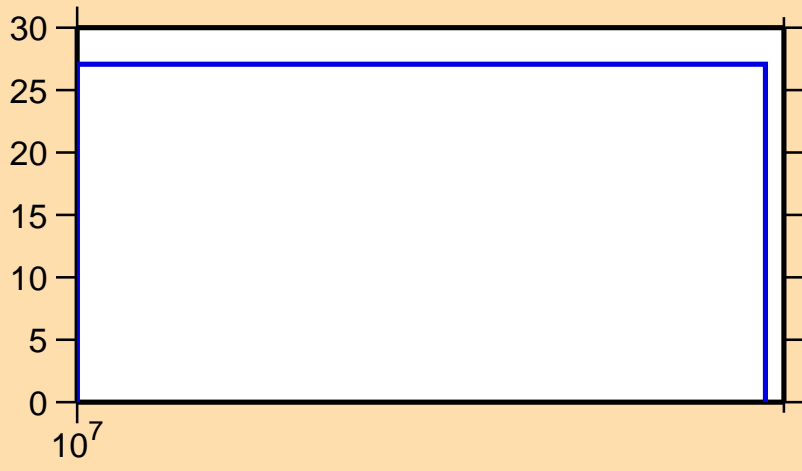
\Delta\sigma/\sigma vs. E for ^{21}\text{O}(n,n_1)
