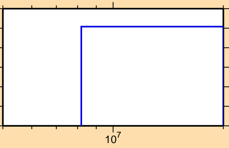
\sigma vs. E for ^{21}\text{O}(n,t)
