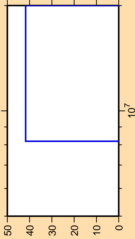
\Delta\sigma/\sigma vs. E for ^{21}\text{O}(n,\alpha)
