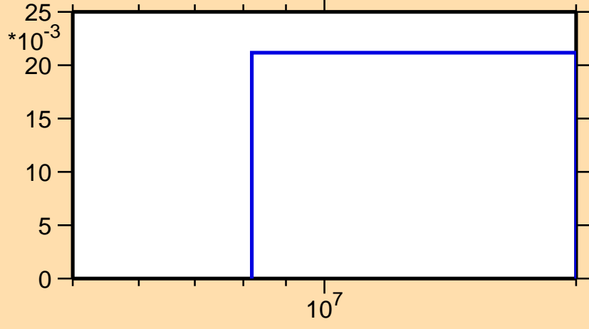
\sigma vs. E for ^{21}\text{O}(n,3n)
