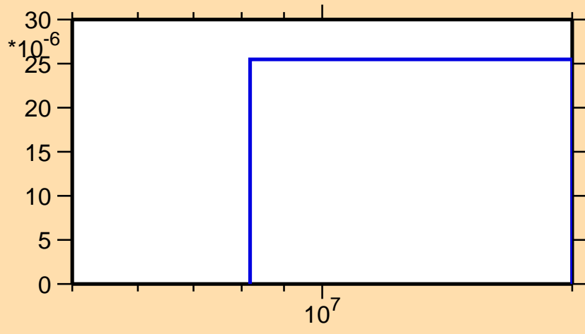
\sigma vs. E for ^{21}\text{O}(n,\alpha)
