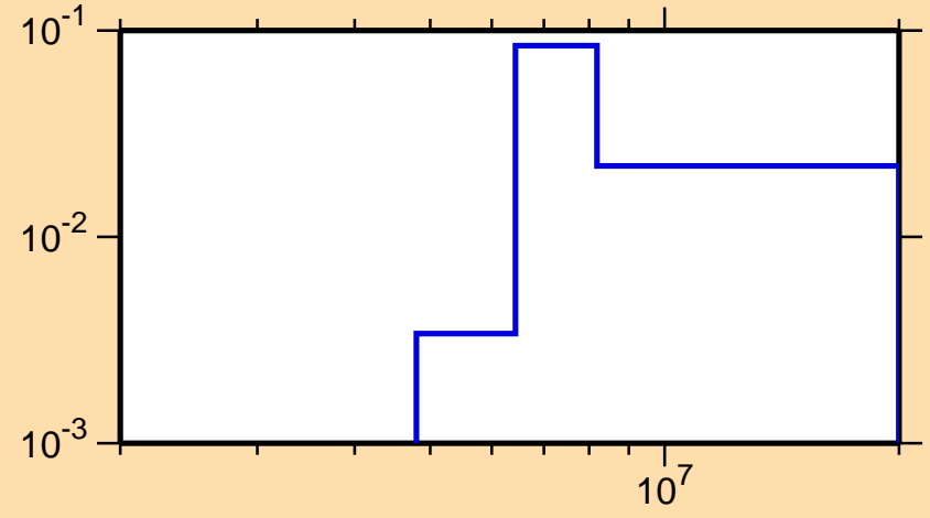
\sigma vs. E for ^{22}\text{O}(n,n_4)
