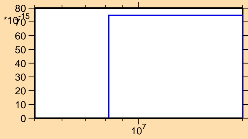
\sigma vs. E for ^{22}\text{O}(n,n\alpha)
