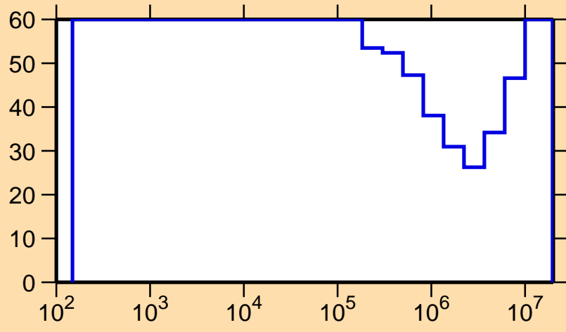
\Delta\sigma/\sigma vs. E for ^{168}\text{Os}(n,p)
