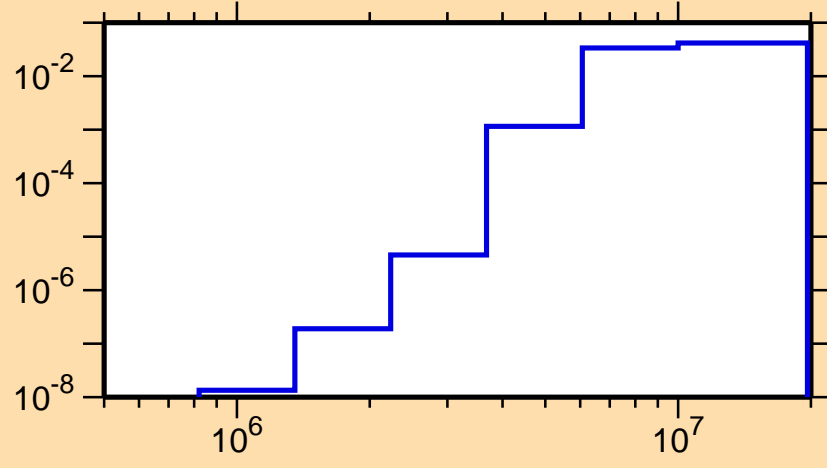
\sigma vs. E for ^{168}\text{Os}(n,n\alpha)
