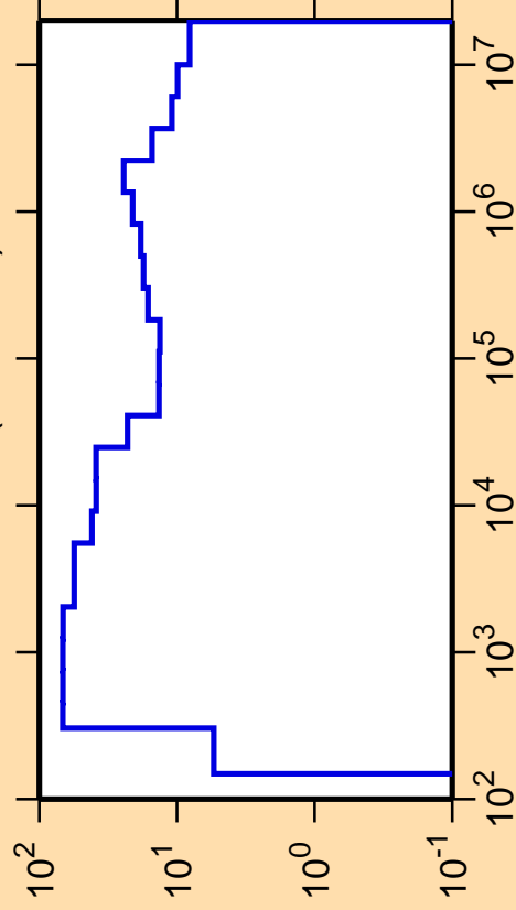
\Delta\sigma/\sigma vs. E for ^{168}\text{Os}(n,\text{nonel.})
