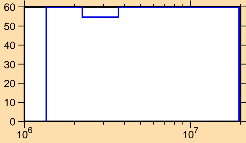
\Delta\sigma/\sigma vs. E for ^{168}\text{Os}(n,n\text{cont.})
