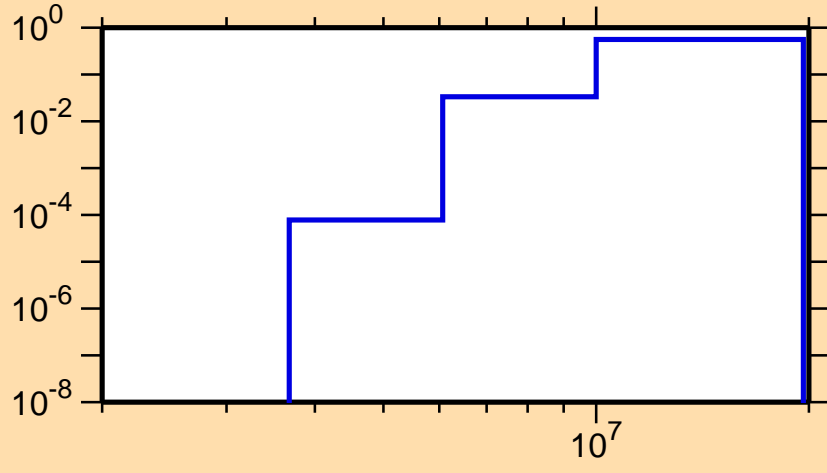
\sigma vs. E for ^{168}\text{Os}(n,np)
