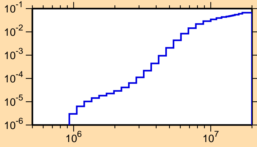
\sigma vs. E for ^{169}\text{Os}(n,n\alpha)
