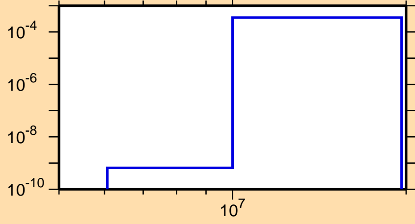
\sigma vs. E for ^{169}\text{Os}(n,t)
