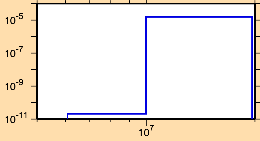
\sigma vs. E for ^{169}\text{Os}(n,\text{pd})
