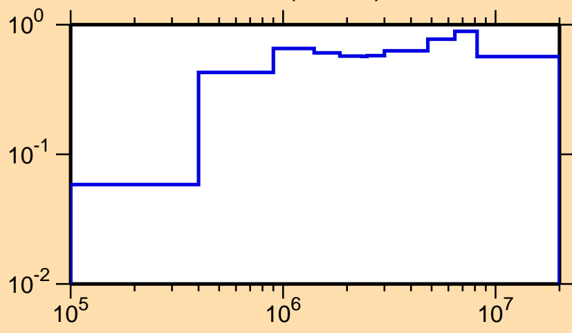
\sigma vs. E for ^{169}\text{Os}(n,\text{inel.})
