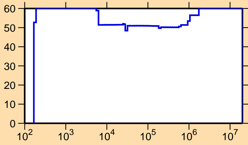
\Delta\sigma/\sigma vs. E for ^{170}\text{Os}(n,\gamma)
