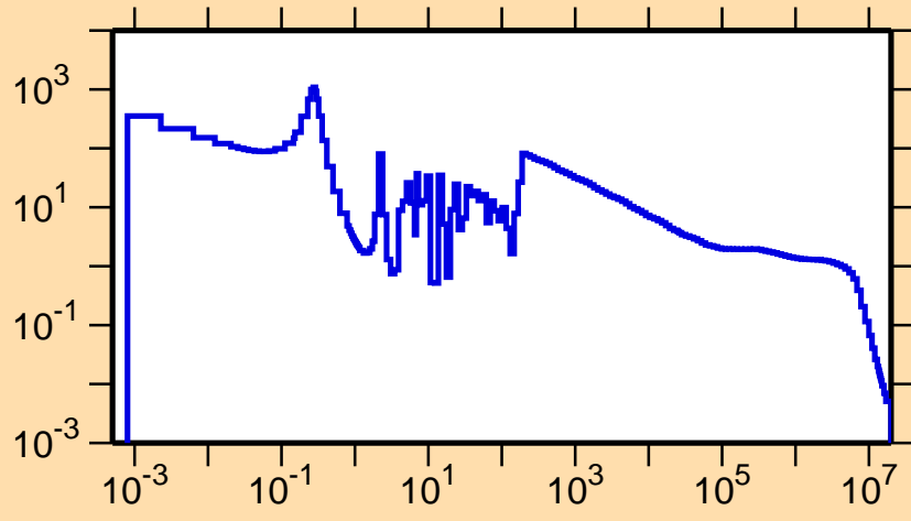
\sigma vs. E for ^{170}\text{Os}(n,\gamma)
