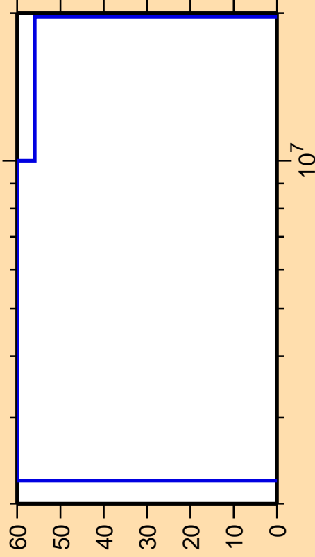
\Delta\sigma/\sigma vs. E for ^{170}\text{Os}(n,n_{\text{cont}}) .
