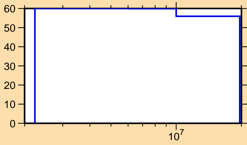
\Delta\sigma/\sigma vs. E for ^{170}\text{Os}(n,n\text{cont.})
