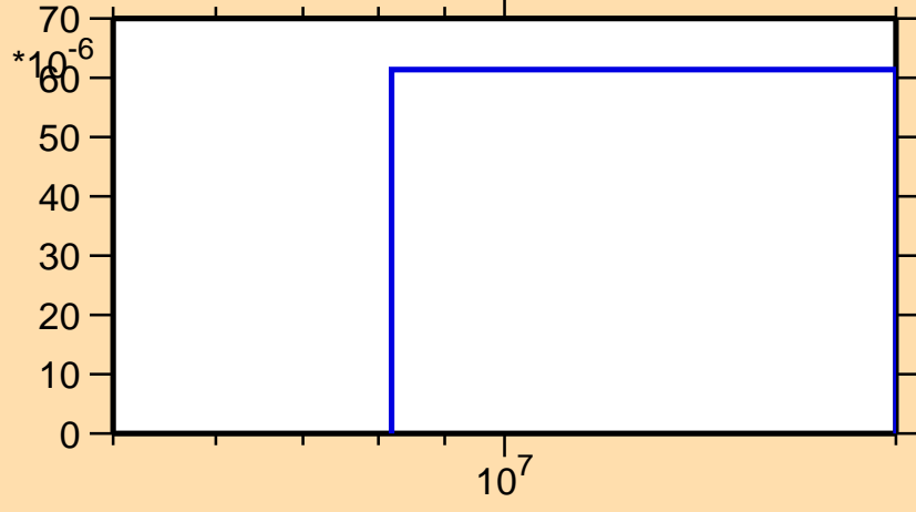
\sigma vs. E for ^{170}\text{Os}(n,t)
