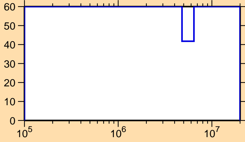
\Delta\sigma/\sigma vs. E for ^{170}\text{Os}(n,n_1)
