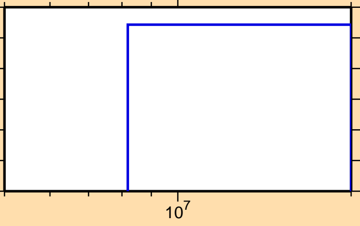
\sigma vs. E for ^{170}\text{Os}(n,2np)
