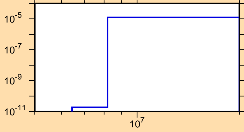
\sigma vs. E for ^{170}\text{Os}(\text{mt117})
