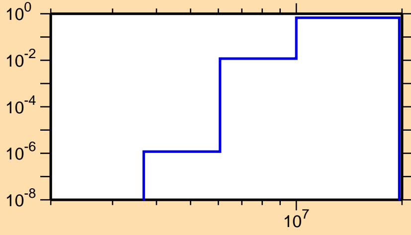
\sigma vs. E for ^{171}\text{Os}(n,np)
