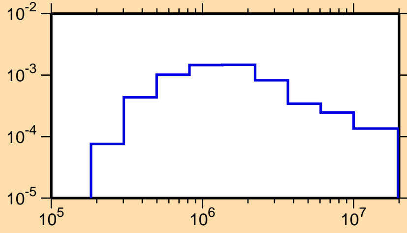
\sigma vs. E for ^{171}\text{Os}(n,n_2)
