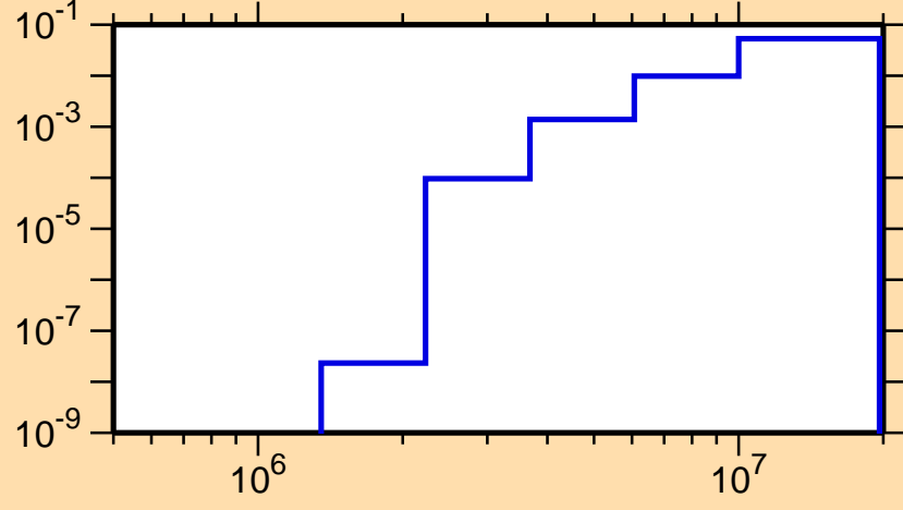
\sigma vs. E for ^{171}\text{Os}(n,n\alpha)
