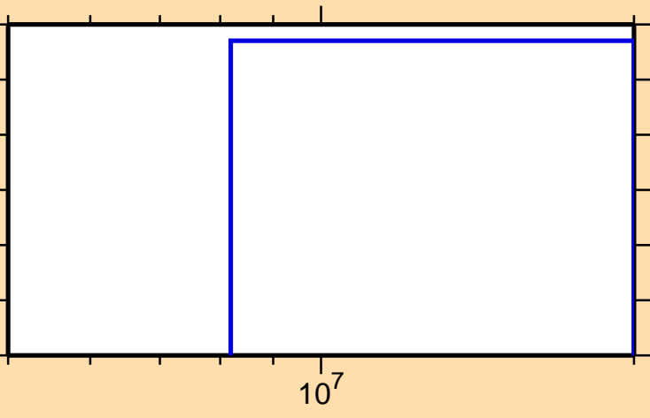
\sigma vs. E for ^{171}\text{Os}(n,3n)
