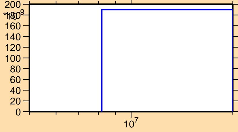
\sigma vs. E for ^{171}\text{Os}(n,\text{nd})
