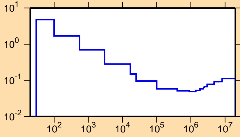
\sigma vs. E for ^{171}\text{Os}(n,\alpha)
