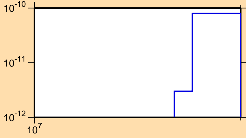
\sigma vs. E for ^{172}\text{Os} (mt 34)
