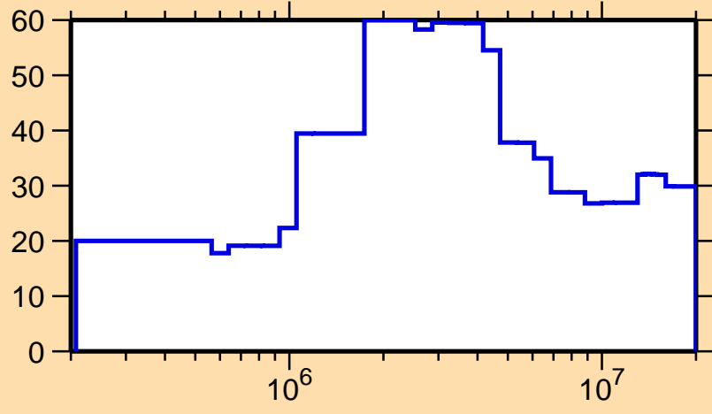
\Delta\sigma/\sigma vs. E for ^{172}\text{Os}(n,\text{inel.})
