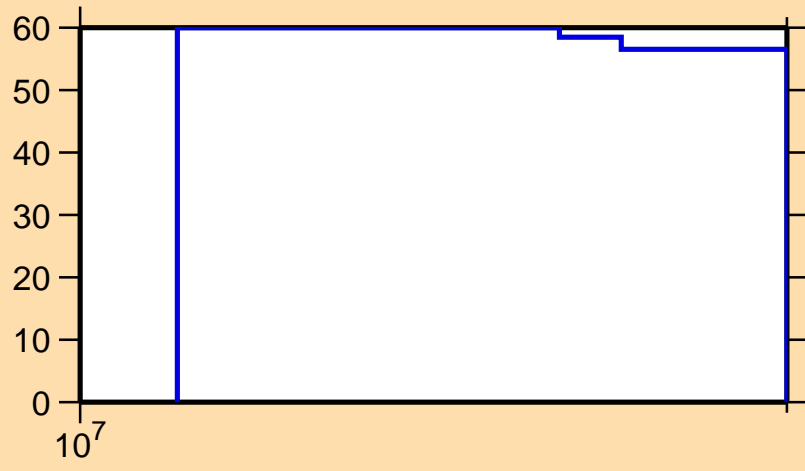
\Delta\sigma/\sigma vs. E for ^{172}\text{Os}(n,2n)
