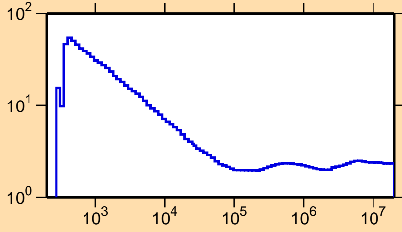
\sigma vs. E for ^{172}\text{Os}(n,\text{nonel.})
