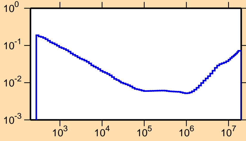
\sigma vs. E for ^{172}\text{Os}(n,\alpha)
