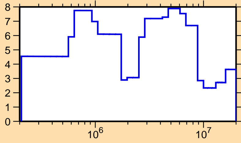
\Delta\sigma/\sigma vs. E for ^{172}\text{Os}(n,\text{tot.})
