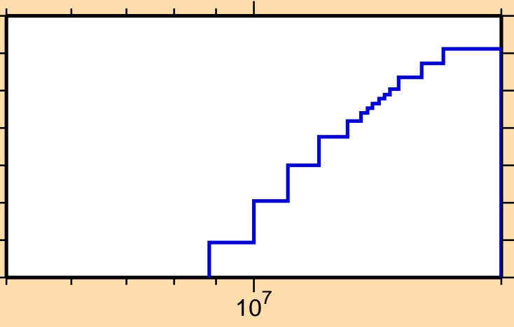
\sigma vs. E for ^{172}\text{Os}(\text{mt117})
