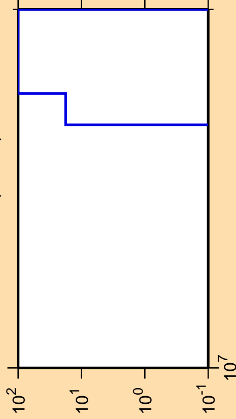
\Delta\sigma/\sigma vs. E for ^{172}\text{Os} (mt 34)
