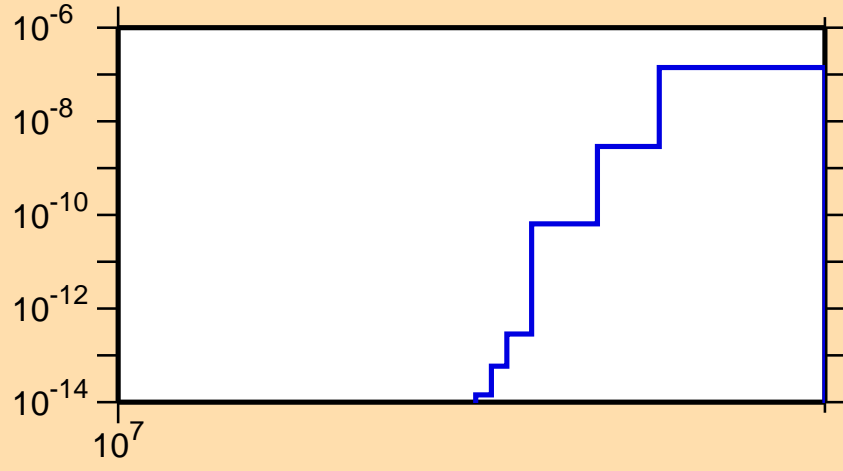
\sigma vs. E for ^{172}\text{Os}(n,\text{nd})
