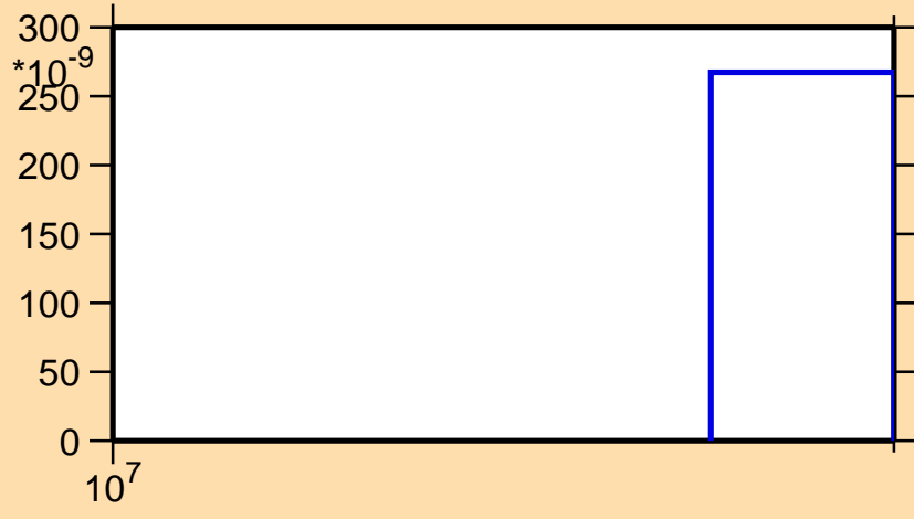
\sigma vs. E for ^{172}\text{Os}(n,3n)
