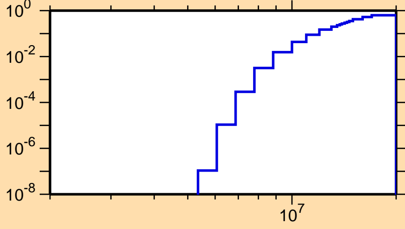
\sigma vs. E for ^{172}\text{Os}(n,np)
