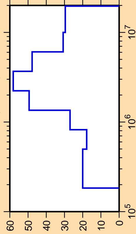
\Delta\sigma/\sigma vs. E for ^{172}\text{Os}(n,\text{inel.})
